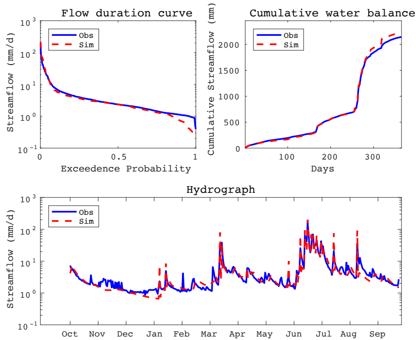
Fig. 7. Combined figures of flow duration curve (top left), cumulative flow (top right) and one-year hydrograph (bottom) in SIM (NSE(Q) = 0.711; NSE(logQ) = 0.647; NSE(FDC) = 0.937; NSE(CF) = 0.996).
