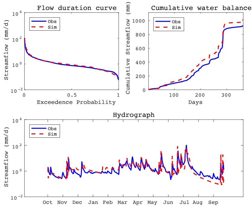
Fig. 3. Combined figures of flow duration curve (top left), cumulative flow (top right) and one-year hydrograph (bottom) in HAZ ( NSE(Q) = 0.209 ; NSE(\log Q) = 0.430 ; NSE(FDC) = 0.894 ; NSE(CF) = 0.965 ).
