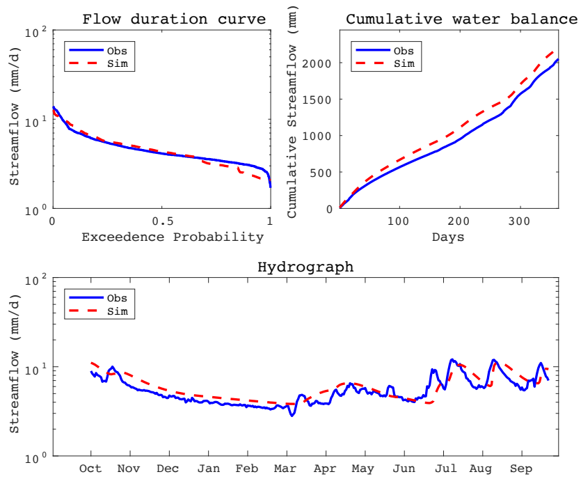
Fig. 8. Combined figures of flow duration curve (top left), cumulative flow (top right) and one-year hydrograph (bottom) in SNK ( NSE(Q) = 0.358 ; NSE(\log Q) = 0.365 ; NSE(FDC) = 0.947 ; NSE(CF) = 0.941 ).
