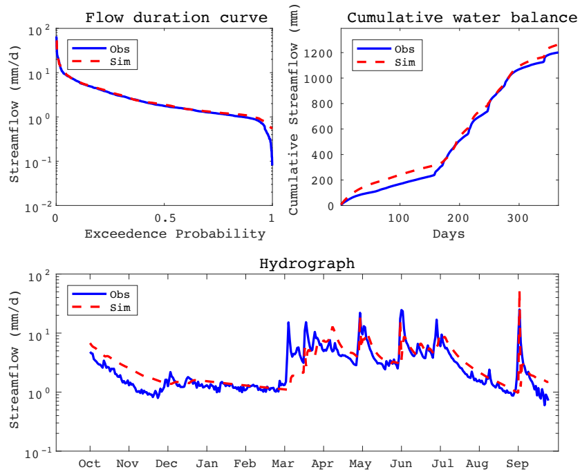
Fig. 4. Combined figures of flow duration curve (top left), cumulative flow (top right) and one-year hydrograph (bottom) in IKR ( NSE(Q) = 0.428 ; NSE(\log Q) = 0.510 ; NSE(FDC) = 0.968 ; NSE(CF) = 0.985 ).
