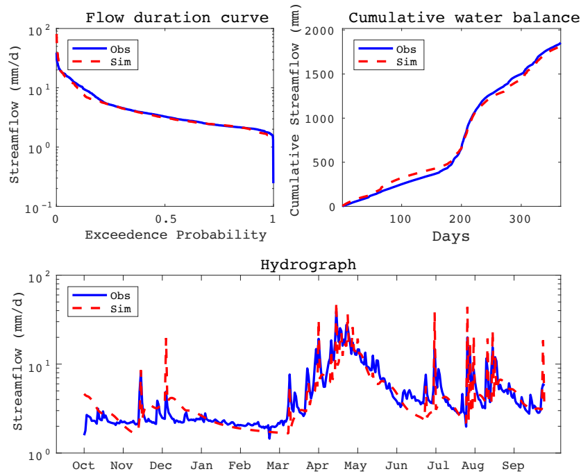
Fig. 2. Combined figures of flow duration curve (top left), cumulative flow (top right) and one-year hydrograph (bottom) in ASE ( NSE(Q) = 0.419 ; NSE(\log Q) = 0.689 ; NSE(FDC) = 0.794 ; NSE(CF) = 0.994 ).
