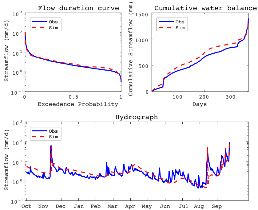
Fig. 5. Combined figures of flow duration curve (top left), cumulative flow (top right) and one-year hydrograph (bottom) in KAM ( NSE(Q) = 0.696 ; NSE(\log Q) = 0.422 ; NSE(FDC) = 0.941 ; NSE(CF) = 0.934 ).
