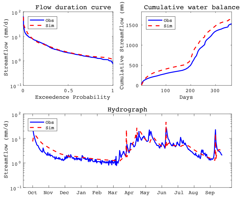
Fig. 6. Combined figures of flow duration curve (top left), cumulative flow (top right) and one-year hydrograph (bottom) in KWM (NSE(Q) = 0.302; NSE(logQ) = 0.613; NSE(FDC) = 0.883; NSE(CF) = 0.916).
