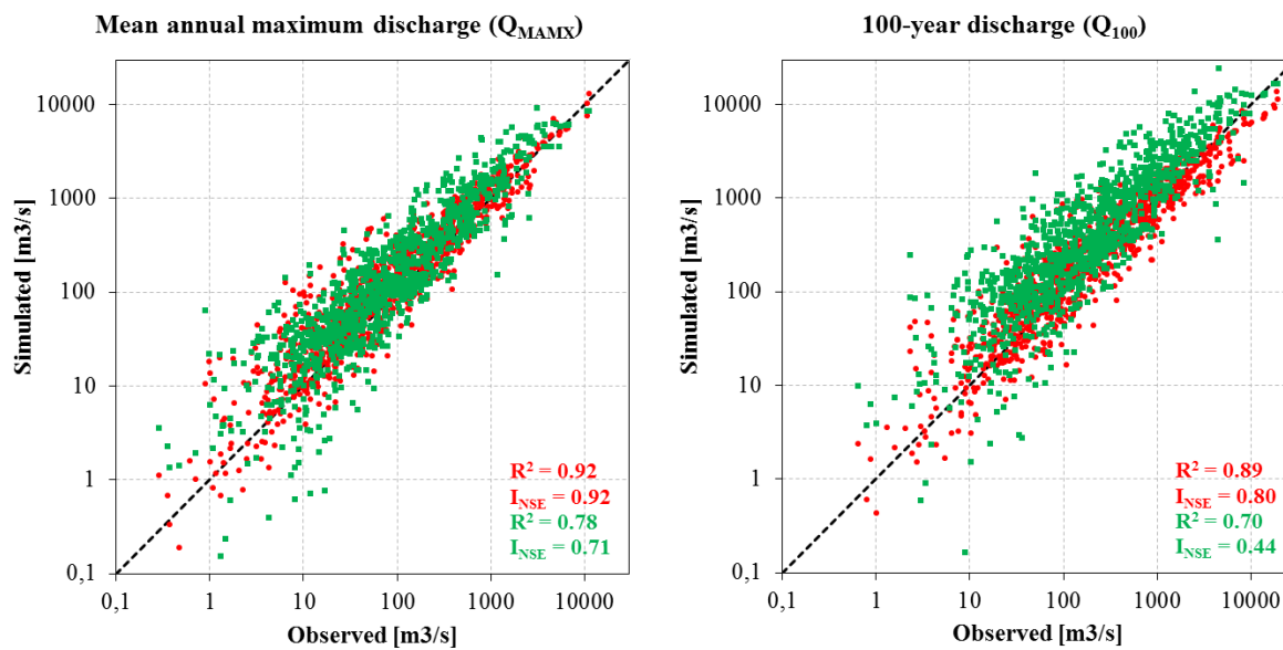
Figure 8. Simulated and observed average annual maxima of daily river discharges and 100-year discharge for 476 stations; Bayesian Network model in red, regional frequency analysis in green. 30-year periods of annual maxima were used (the most recent available out of 1971–2000, 1961–1990 or 1951–1980).
