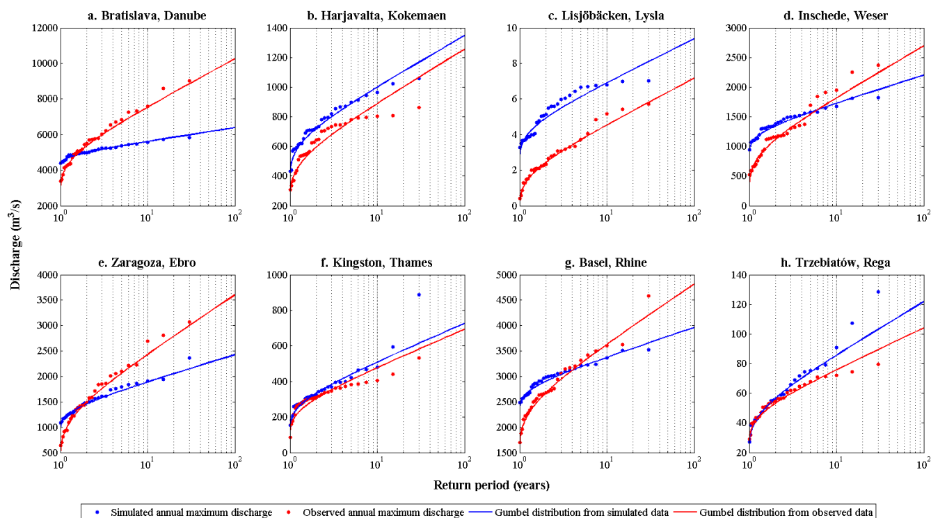
Figure 6. Simulated and observed annual maxima of daily river discharges fitted to Gumbel distribution at selected stations. Data refer to 1971–2000, except h), which refers to 1961–1990.
