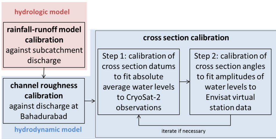
5 Figure 3: Flow chart showing the hydrological and hydrodynamic model calibration.
