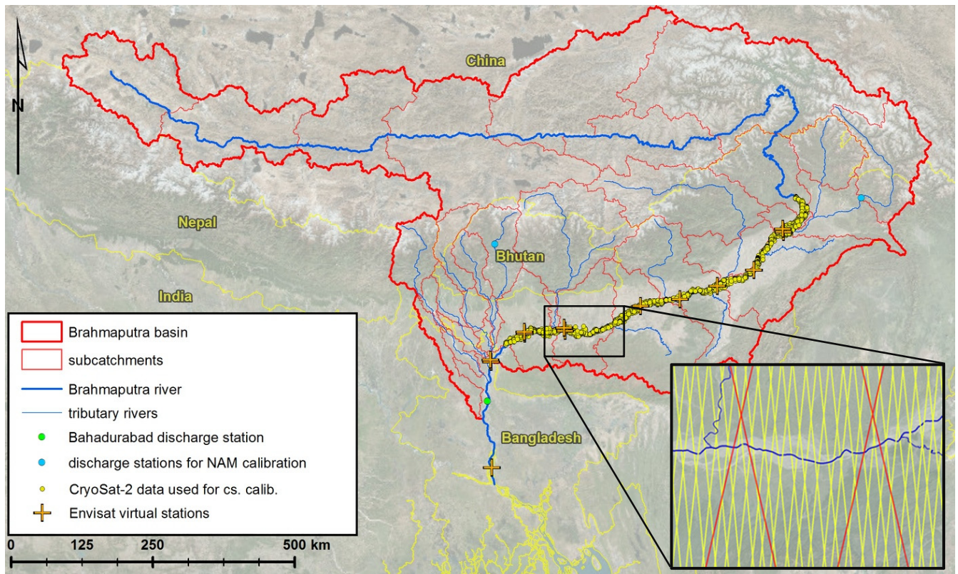
5 | Figure 1: Brahmaputra basin model base map, showing the altimetry data used for the water level calibration (the entire upstream part of the Brahmaputra is also covered by the SARIn mode of CryoSat-2). Map inset: Ground tracks of CryoSat-2 (yellow) and Envisat (red). The Brahmaputra River originates in the Tibetan Plateau, flows eastwards, then bends towards south to cross the Himalayan Mountains and afterwards flows westwards through the Assam Valley into Bangladesh.
