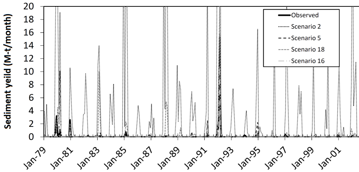
Figure 10. Simulated and observed monthly sediment yield (M-t/month) for scenarios 2, 5, 18 and 16.
