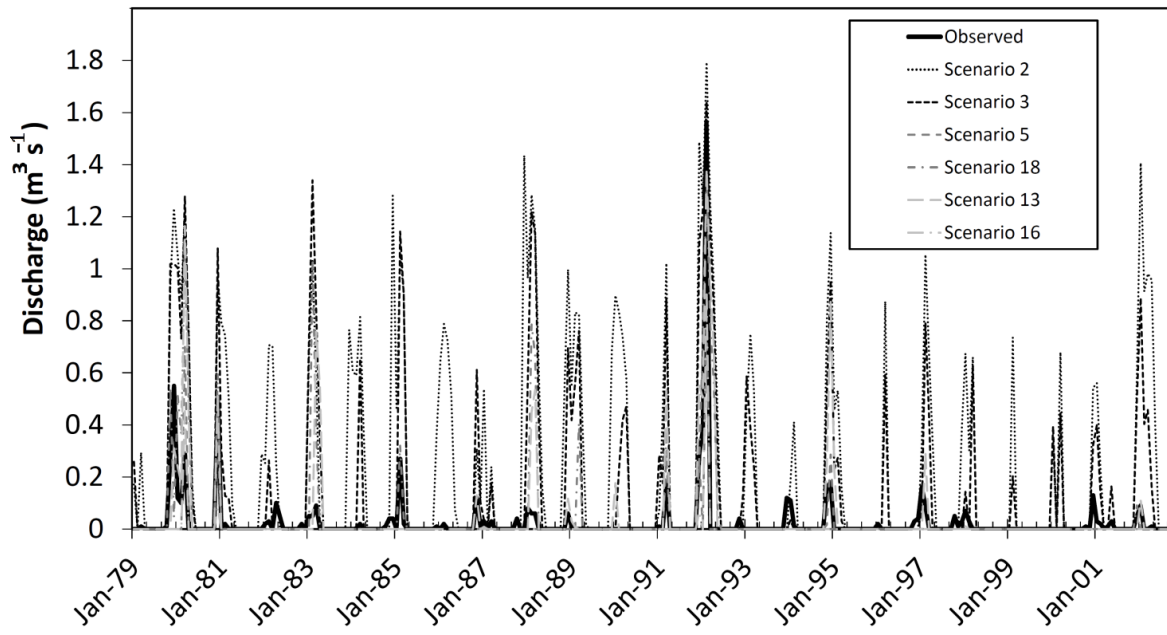
Figure 9. Simulated and observed average monthly discharge (m 3 s -1 ) for scenarios 2, 3, 5, 18, 13 and 16.
