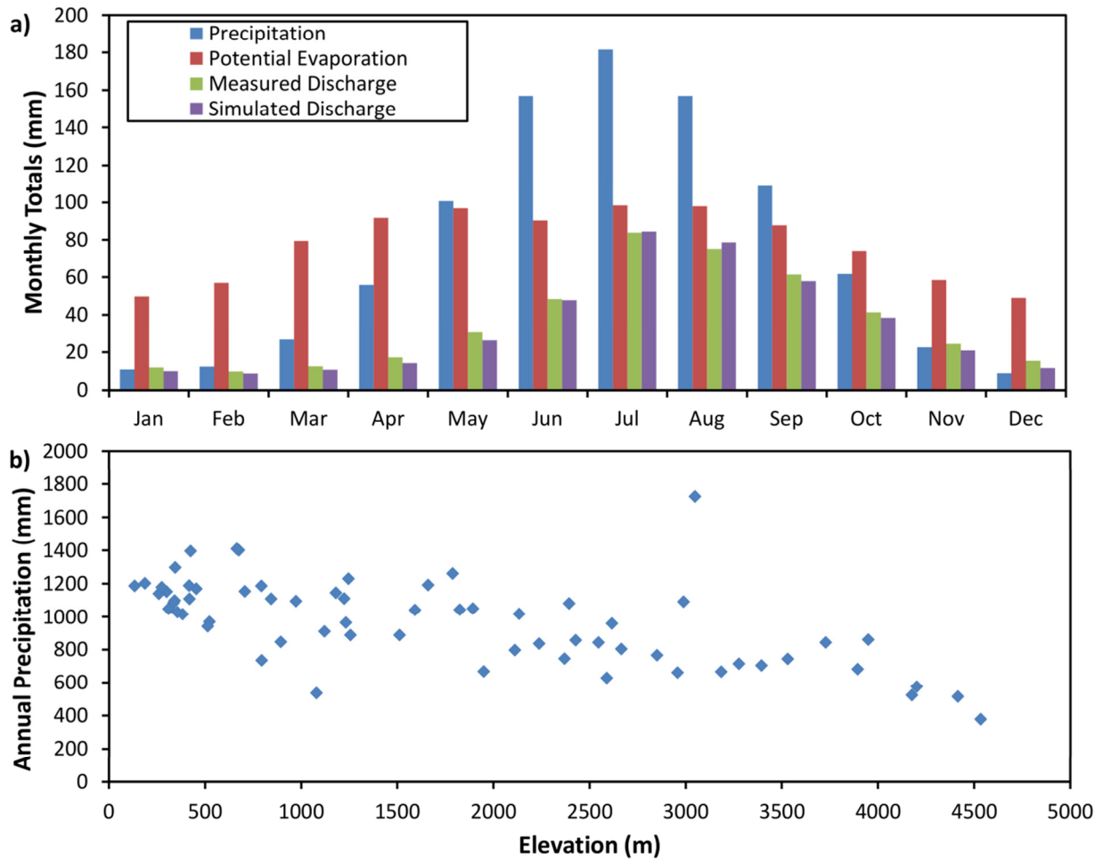
Figure 2. (a) Monthly precipitation, potential evaporation, measured and simulated discharge totals in the Yangtze basin to Yichang, 1996-2005.(b) Comparison of the elevation of the precipitation station and the annual precipitation totals
