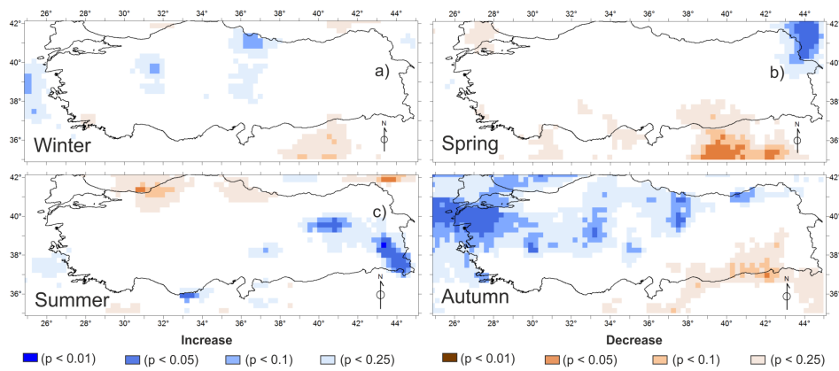
Fig. 6. The presence and the direction of Total Precipitation trends by InterimLand for a) Winter, b) Spring, c) Summer and d) Autumn
