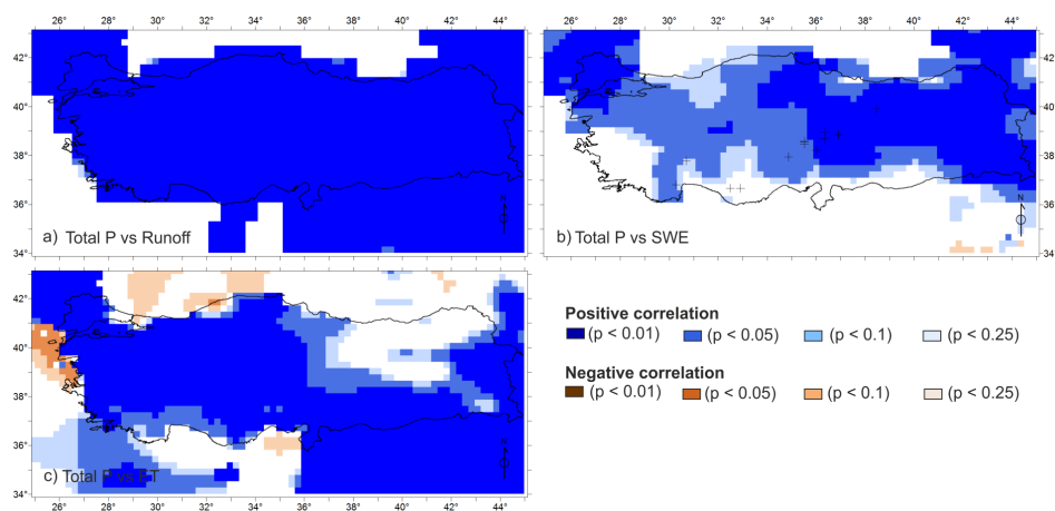
Fig. 8. The correlation between (a) total Precipitation and Runoff, (b) total Precipitation and SWE, (c) total Precipitation and ET for InterimLand dataset
