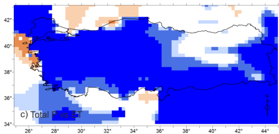
Fig. 10. Fig9b The correlationbetween totalP and ET
