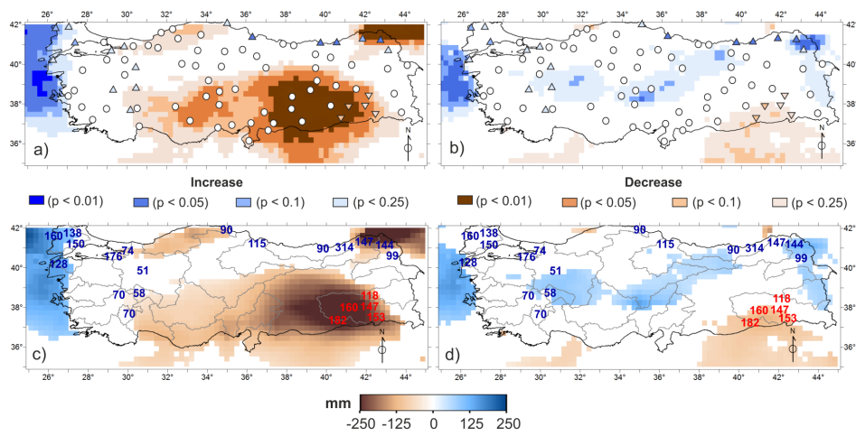
Fig. 6. Fig6 TotalP trends vs stations
