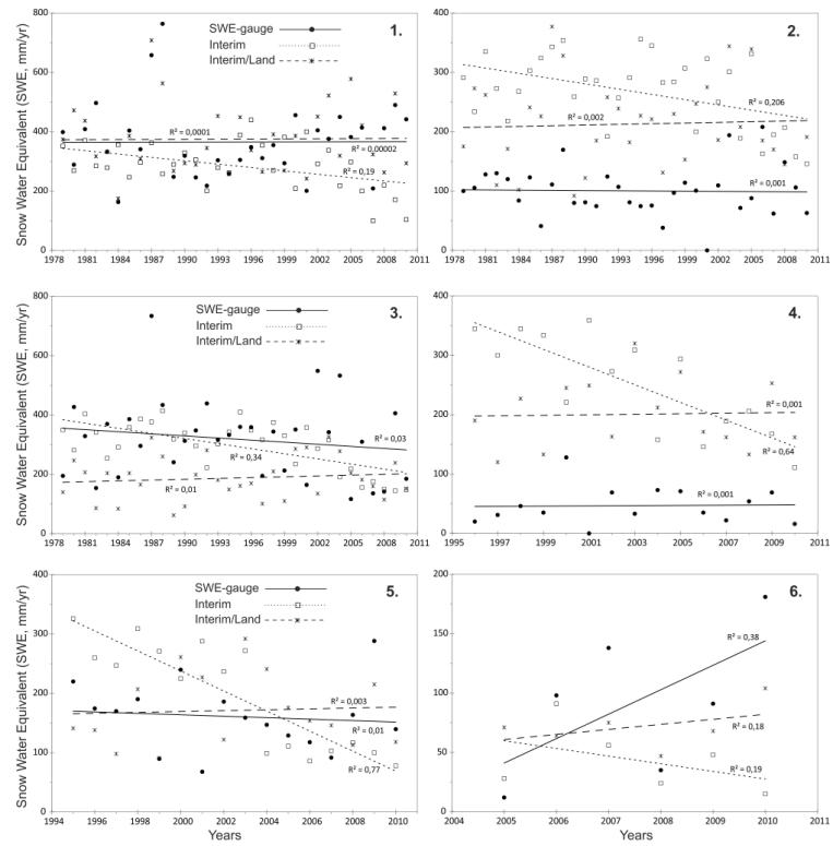
Fig. 8. Fig7.2 SWE comparison with stations
