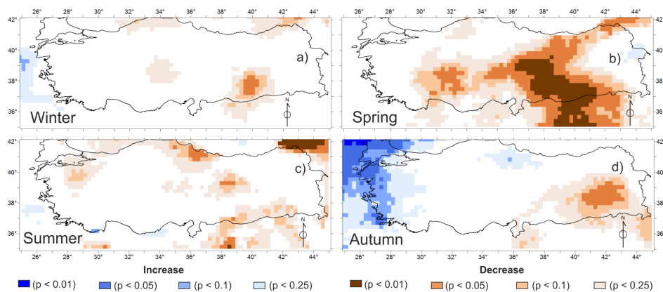
Fig. 1. Fig1 ERA-I totalP seasonal trends (significance)
