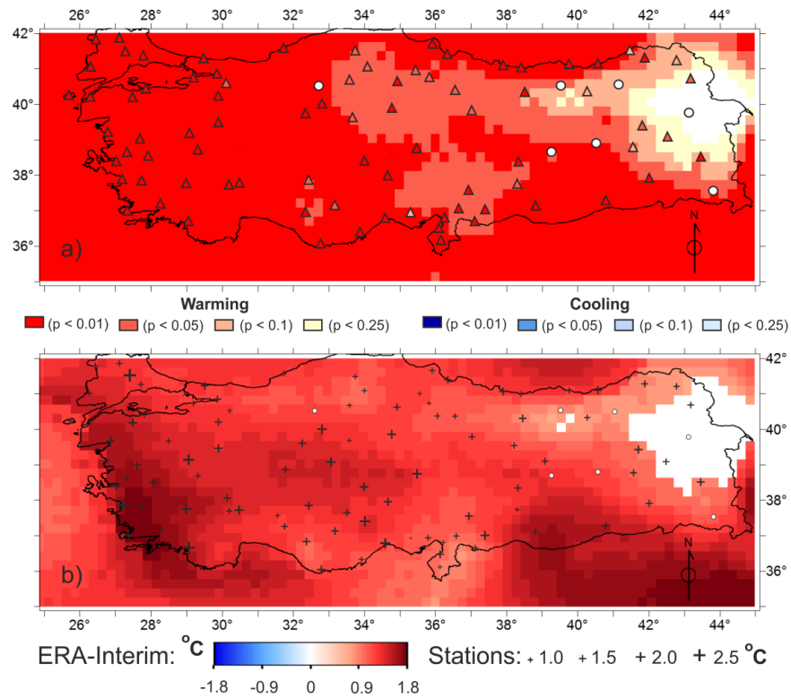
Fig. 5. Fig5 T2m trends (revised)
