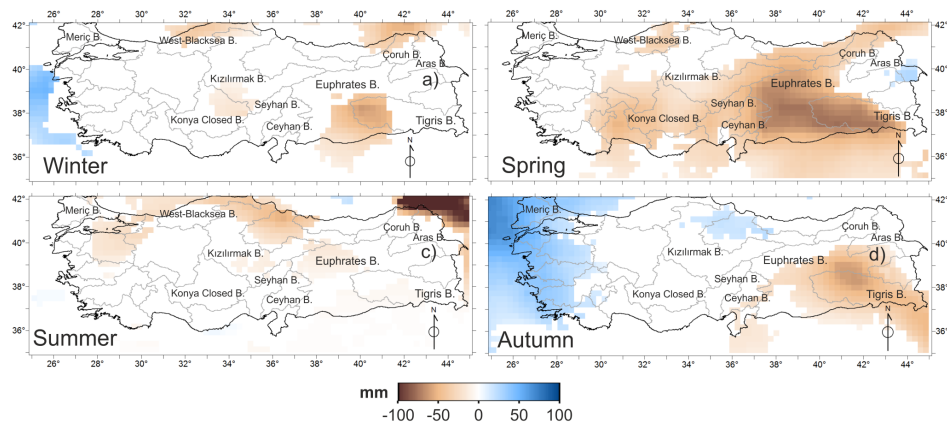
Fig. 2. Fig2 ERA-I totalP seasonal trends (magnitude)
