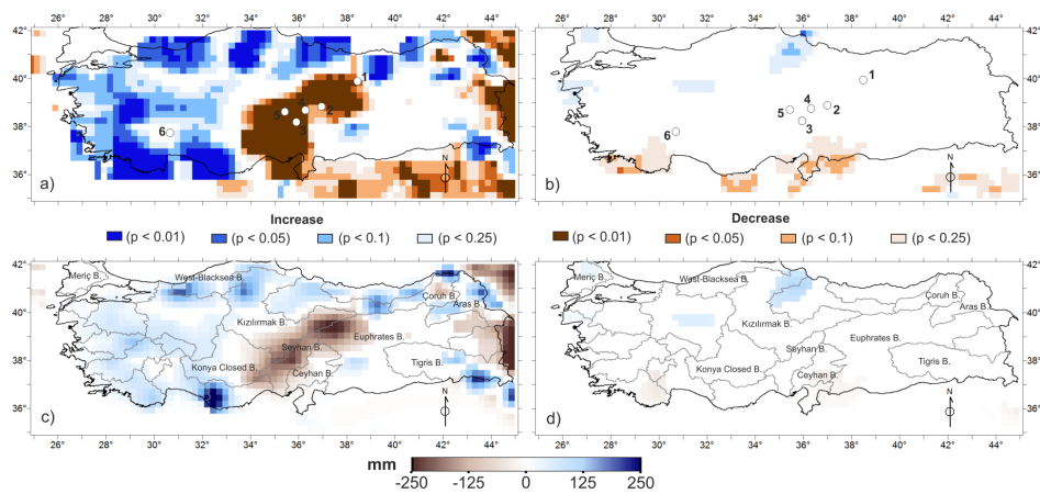
Fig. 7. Fig7.1 SWE trends (revised)
