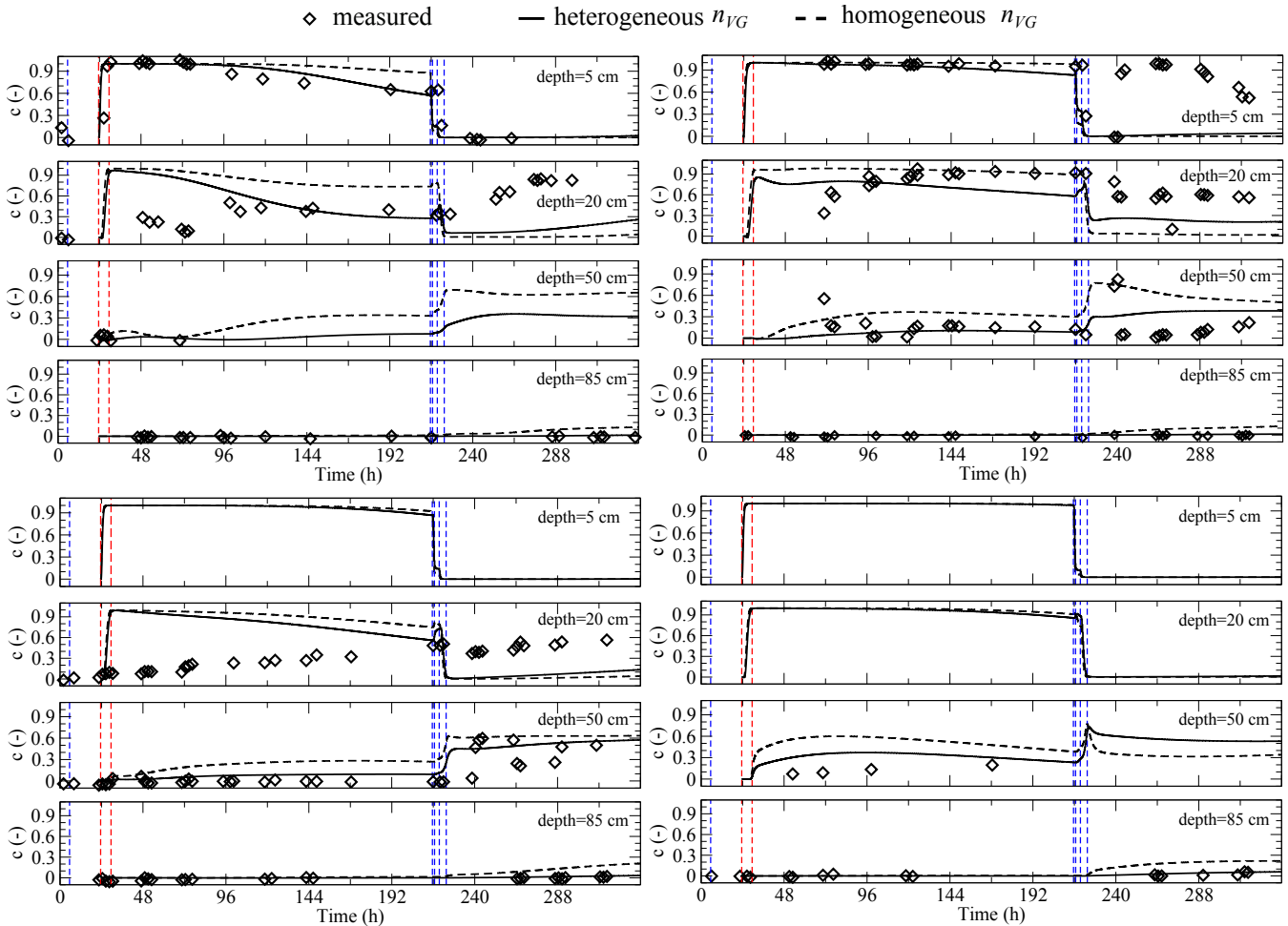
Figure 12. Distributed (internal state) hydrological response for the tracer concentration breakthrough curves at 5, 20, 50, and 85 cm depth from the surface for four locations on the LEO-1 hillslope: point a (top left), point b (top right), point c (bottom left), and point d (bottom right) of Fig. 2. There were no tracer concentration measurements at 5 cm depth for point c and at 5 and 20 cm depth for point d. The transport model is run for \alpha_t=0.001 m and \alpha_t=0.0001 m. The vertical dashed lines indicate the timing of the three pulses of rain (red when the water is ^2H -enriched and blue when it is not).
