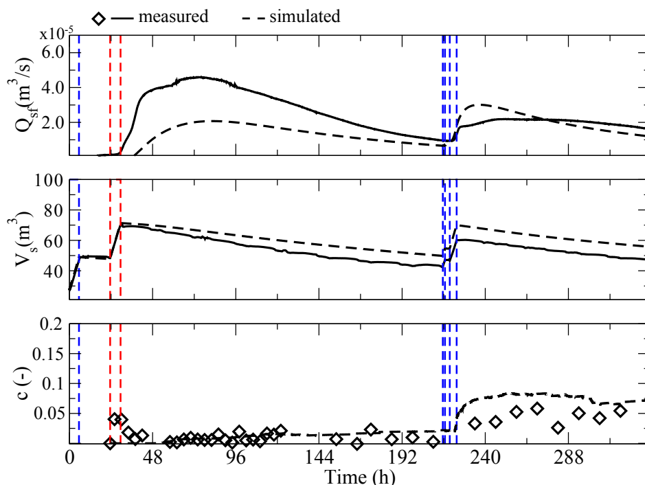
Figure 13. Performance of the model against integrated flow and transport responses (seepage face flow Q_{sf} , total water storage V_s , and average tracer concentration c at the seepage face) using the additional parameterization from the distributed analyses (spatially variable soil retention capacity). The vertical dashed lines indicate the timing of the three pulses of rain (red when the water is ^2H -enriched and blue when it is not).
