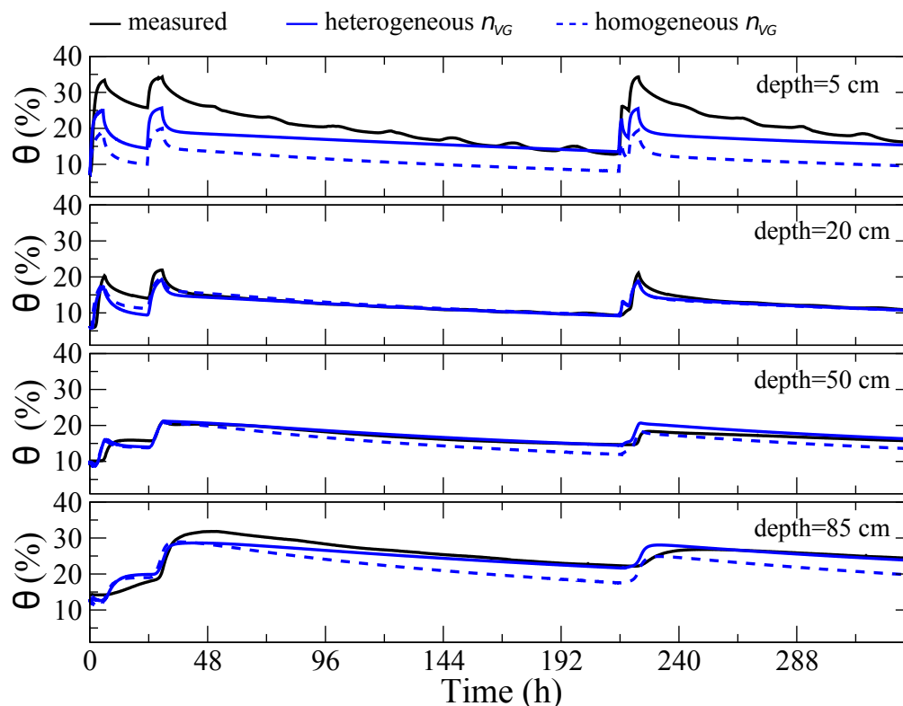
Figure 10. Averaged \theta profiles at 5, 20, 50, and 85 cm depth from the surface.
