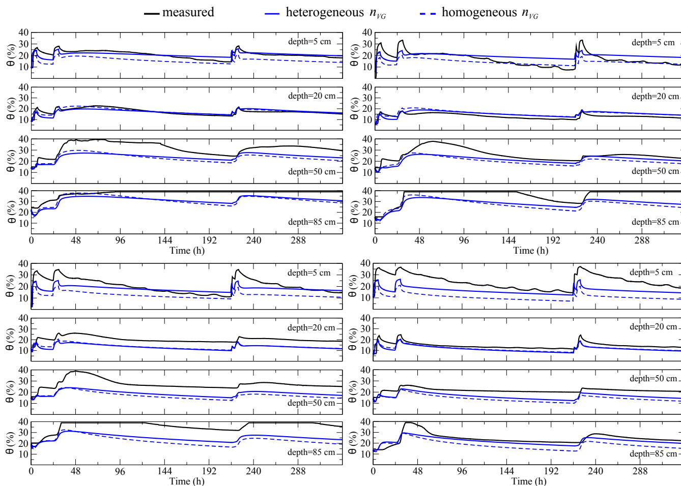
Figure 11. Distributed (internal state) hydrological response for the \theta profiles at 5, 20, 50, and 85 cm depth from the surface for four locations on the LEO-1 hillslope: point a (top left), point b (top right), point c (bottom left), and point d (bottom right) of Fig. 2.
