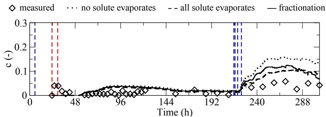
Figure 8. Measured and modeled average tracer concentration at the seepage face for the cases in which no solute, all solute, and some solute (fractionation) leaves the system with evaporation. The three simulations are run for \alpha_l=0.001 m and \alpha_t=0.0001 m. The vertical dashed lines indicate the timing of the three pulses of rain (red when the water is ^2H -enriched and blue when it is not).
