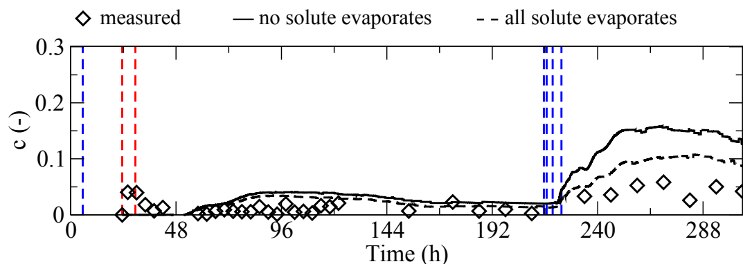
Figure 6. Measured and modeled average tracer concentration at the seepage face for the cases in which no solute and all solute leaves the system with evaporation. Both simulations are run for \alpha_l=0.001 m and \alpha_t=0.0001 m. The vertical dashed lines indicate the timing of the three pulses of rain (red when the water is ^2H -enriched and blue when it is not).
