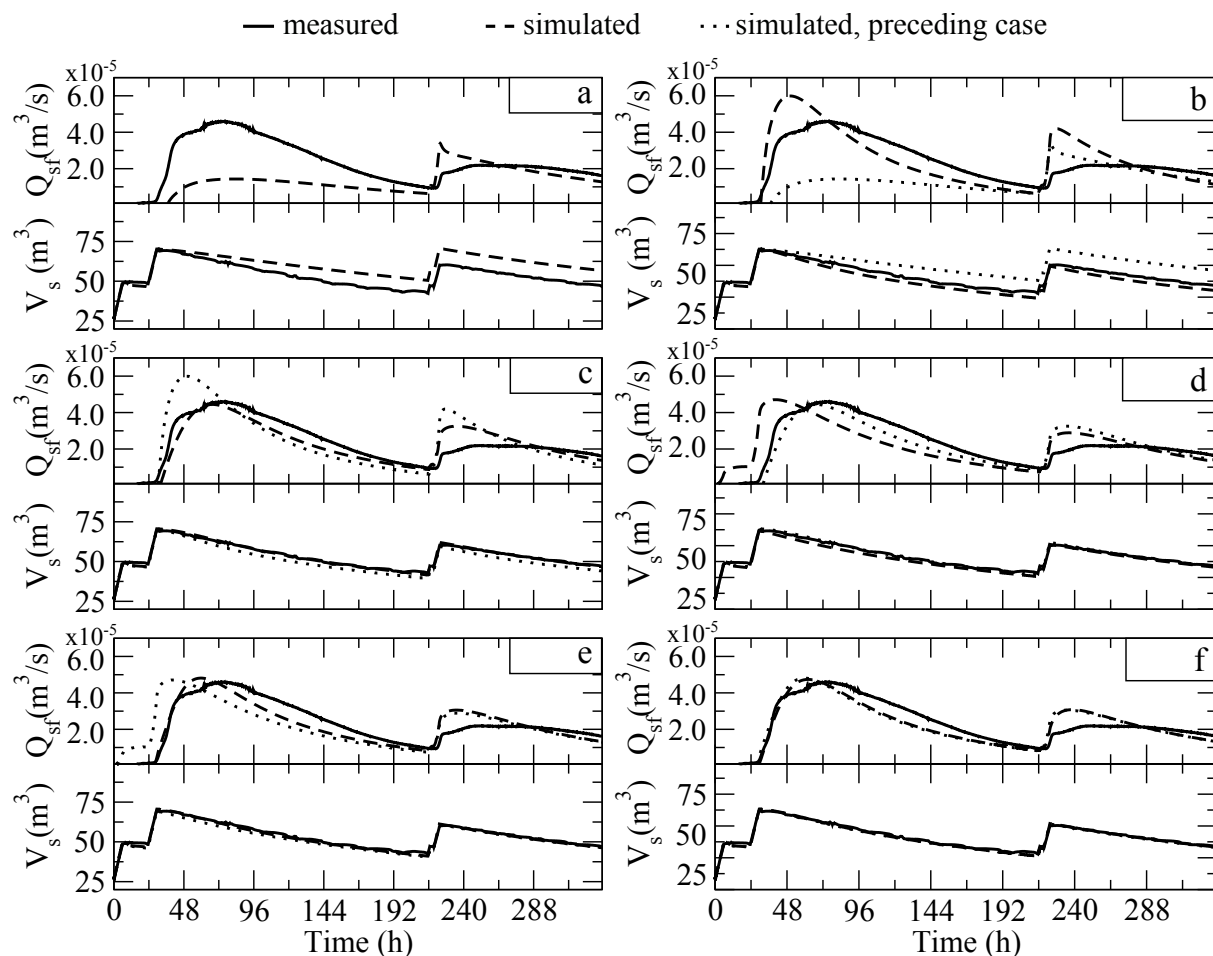
Figure 3. Results for the 6 simulations of the integrated flow response analysis (see Table 3). For each case the seepage face flow Q_{sf} (top) and total water storage V_s (bottom) are reported.
