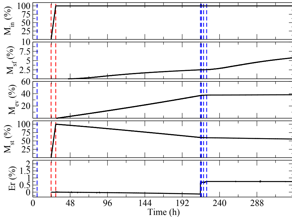
Figure 9. Simulated mass balance results for \alpha_l=0.001 m when the source term f_c is added to the transport equation to perform isotopic fractionation. From top to bottom: ^2H mass that enters the system, M_{in} (normalized with respect to the total mass added to the system during the simulation); that exits through the seepage face, M_{sf} ; that exits through evaporation, M_{ev} ; and that remains in storage, M_{st} . The bottom graph shows the cumulative mass balance error E_r=(M_{in} - M_{sf} - M_{ev} - M_{st}) . The vertical dashed lines indicate the timing of the three pulses of rain (red when the water is ^2H -enriched and blue when it is not).
