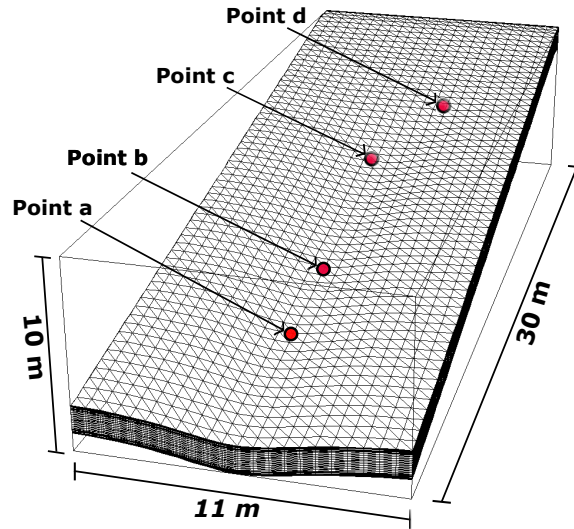
Figure 2. 3D numerical grid for the LEO landscape. Points a, b, c, and d are the locations where samples were extracted during the experiment for subsequent laboratory analysis.
