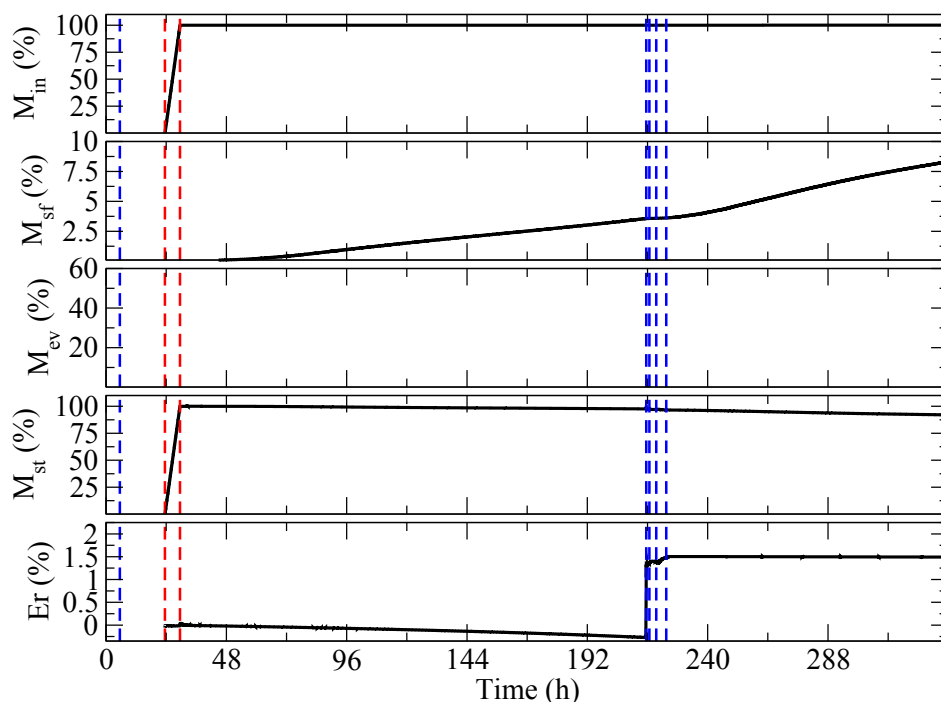
Figure 7. Simulated mass balance results for \alpha_l=0.001 m when the sink term is used to perform evaporation and the correction term f_c added to the transport equation is used to force all the isotopic mass to stay in the system. From top to bottom: ^2H mass that enters the system, M_{in} (normalized with respect to the total mass added to the system during the simulation); that exits through the seepage face, M_{sf} ; that exits through evaporation, M_{ev} ; and that remains in storage, M_{st} . The bottom graph shows the cumulative mass balance error Er=(M_{in} - M_{sf} - M_{ev} - M_{st}) . The vertical dashed lines indicate the timing of the three pulses of rain (red when the water is ^2H -enriched and blue when it is not).
