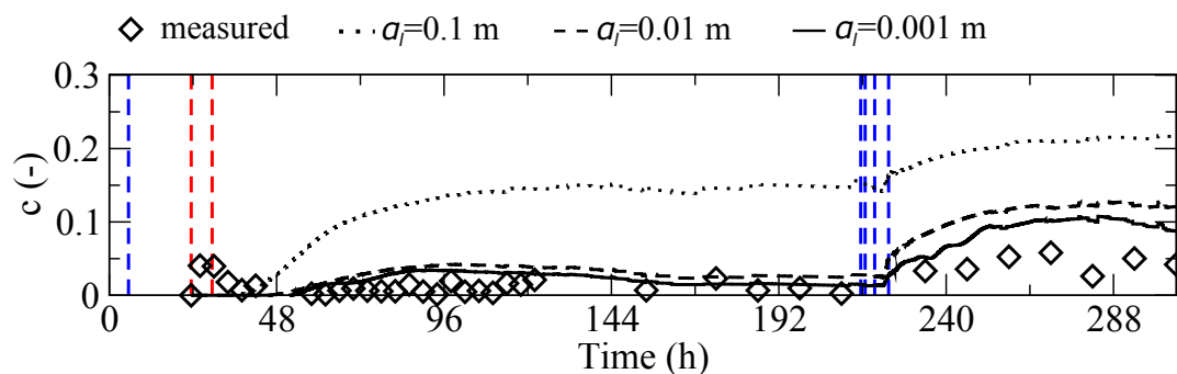
Figure 4. Results for the integrated transport response analysis for different values of dispersivity. The vertical dashed lines indicate the timing of the three pulses of rain (red when the water is ^2H -enriched and blue when it is not).
