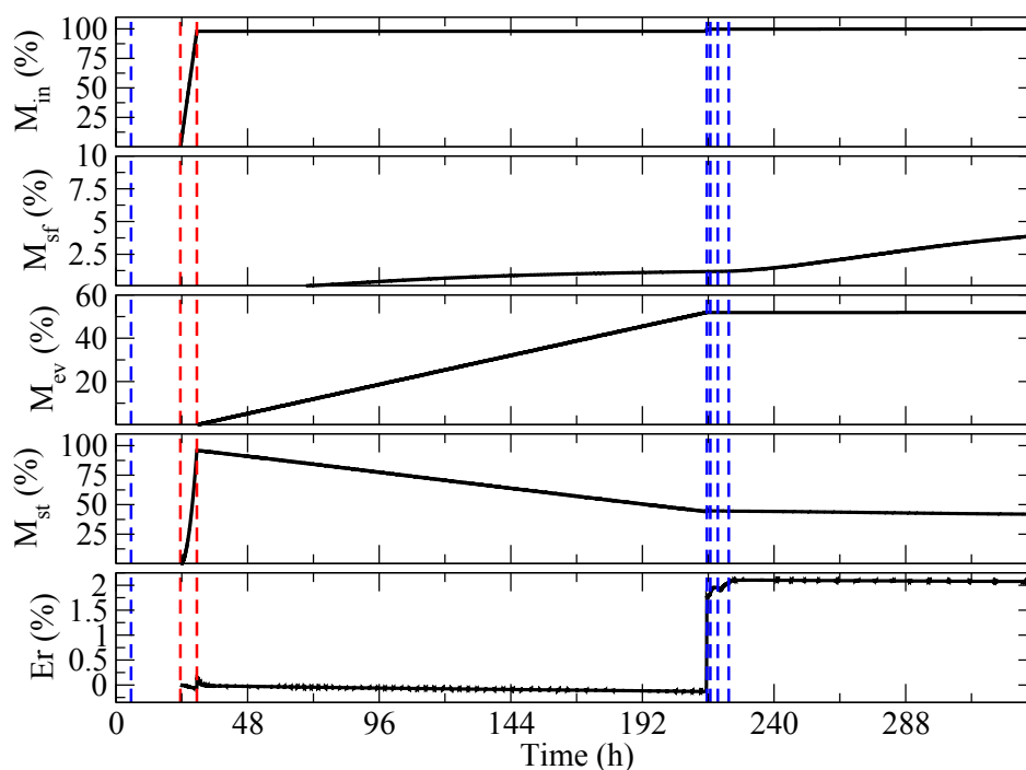
Figure 5. Simulated mass balance results for \alpha_l=0.001 m. From top to bottom: ^2H mass that enters the system, M_{in} (normalized with respect to the total mass added to the system during the simulation); that exits through the seepage face, M_{sf} ; that exits through evaporation, M_{ev} ; and that remains in storage, M_{st} . The bottom graph shows the cumulative mass balance error E_r=(M_{in} - M_{sf} - M_{ev} - M_{st}) . The vertical dashed lines indicate the timing of the three pulses of rain (red when the water is ^2H -enriched and blue when it is not).
