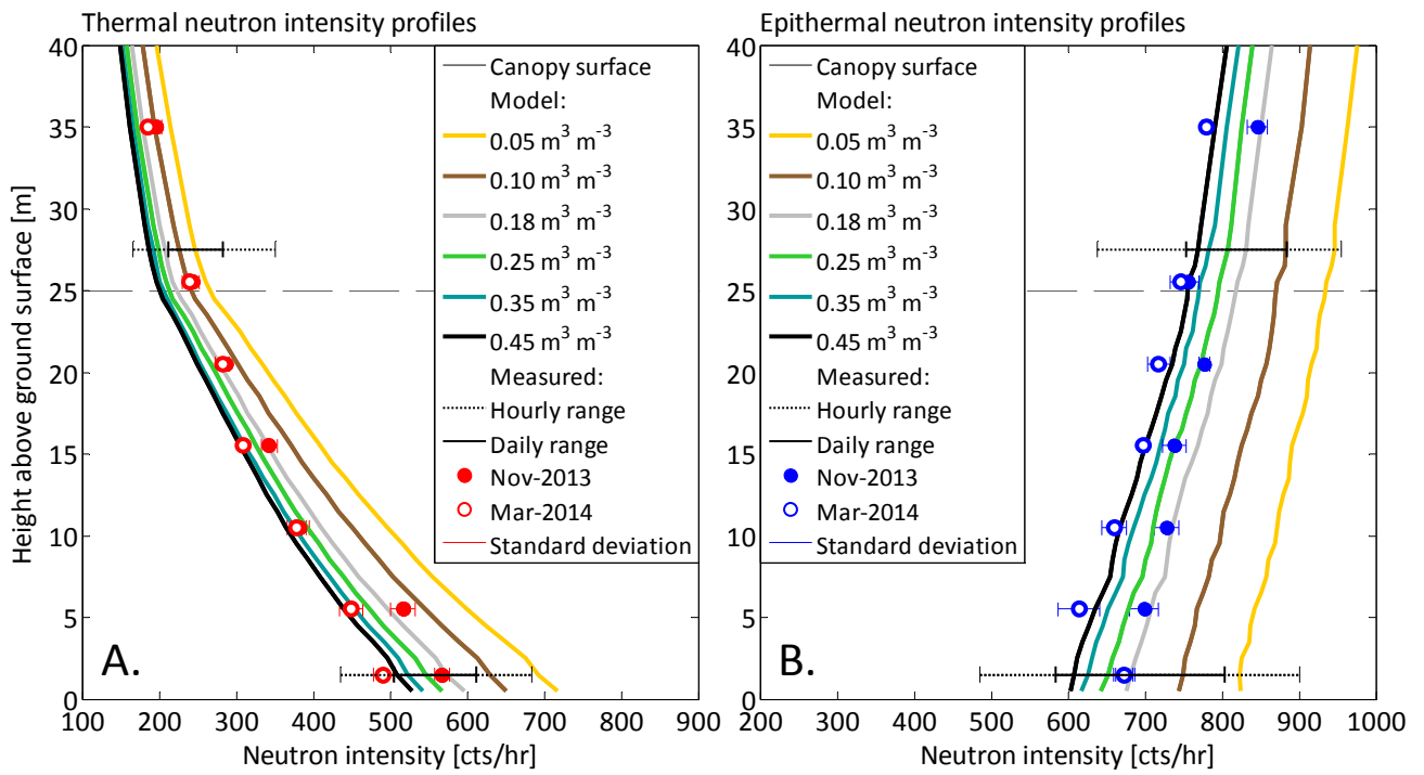
Figure 5 - Sensitivity to volumetric soil moisture using Model Foliage . Measured and modeled (A) thermal and (B) epithermal neutron intensity profiles at Gludsted Plantation. Hourly and daily ranges of variation of thermal and epithermal neutron intensities at ground and canopy level for the period 2013–2015.
