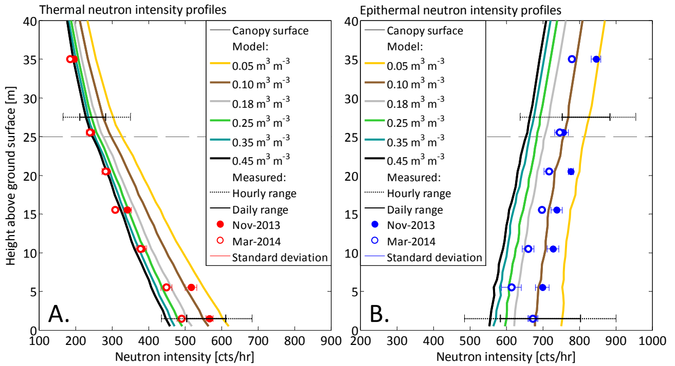
Figure 4 – Sensitivity to volumetric soil moisture using Model Tree trunk, Foliage, Air . Measured and modeled (A) thermal and (B) epithermal neutron intensity profiles at Gludsted Plantation. Hourly and daily ranges of variation of thermal and epithermal neutron intensities at ground and canopy level for the period 2013–2015.
