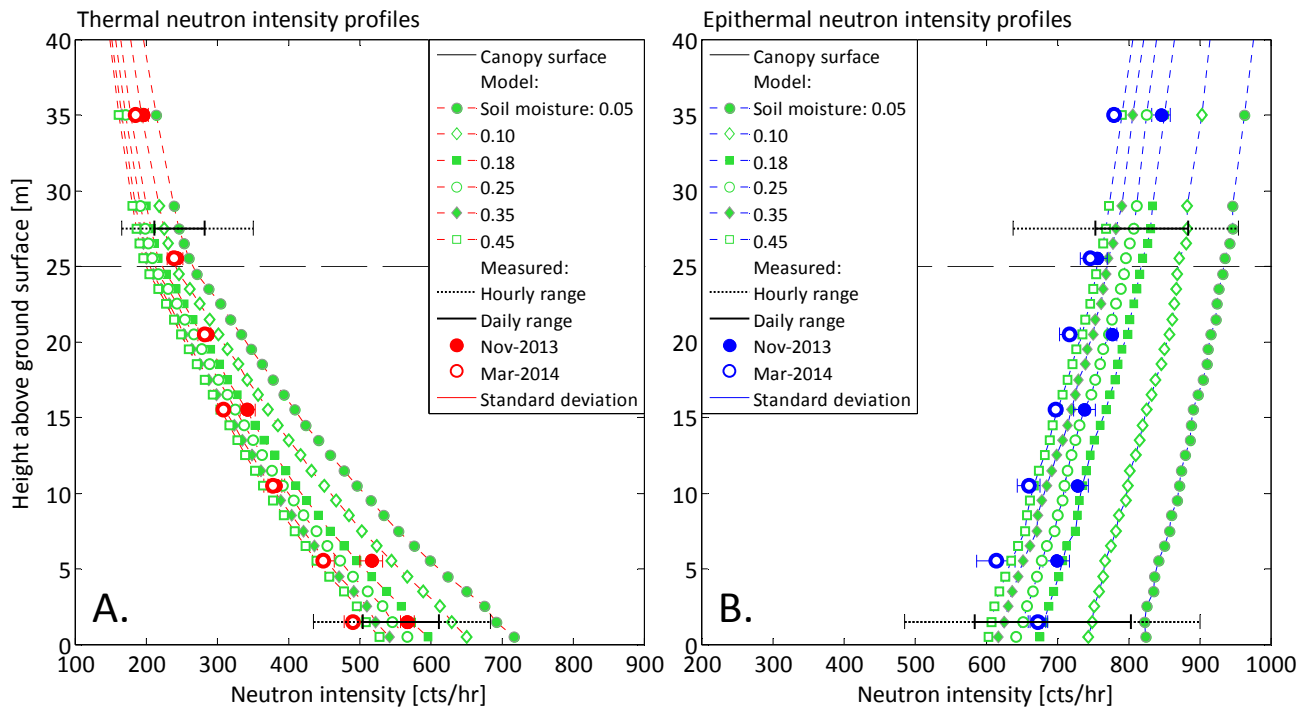
Figure 5 - Sensitivity to volumetric soil moisture, in \text{m}^3 \text{m}^{-3} (Model Foliage ). Measured and modeled (A) thermal and (B) epithermal neutron intensity profiles at Gludsted Plantation. Hourly and daily ranges of variation of thermal and epithermal neutron intensities at ground and canopy level for the period 2013–2015.
