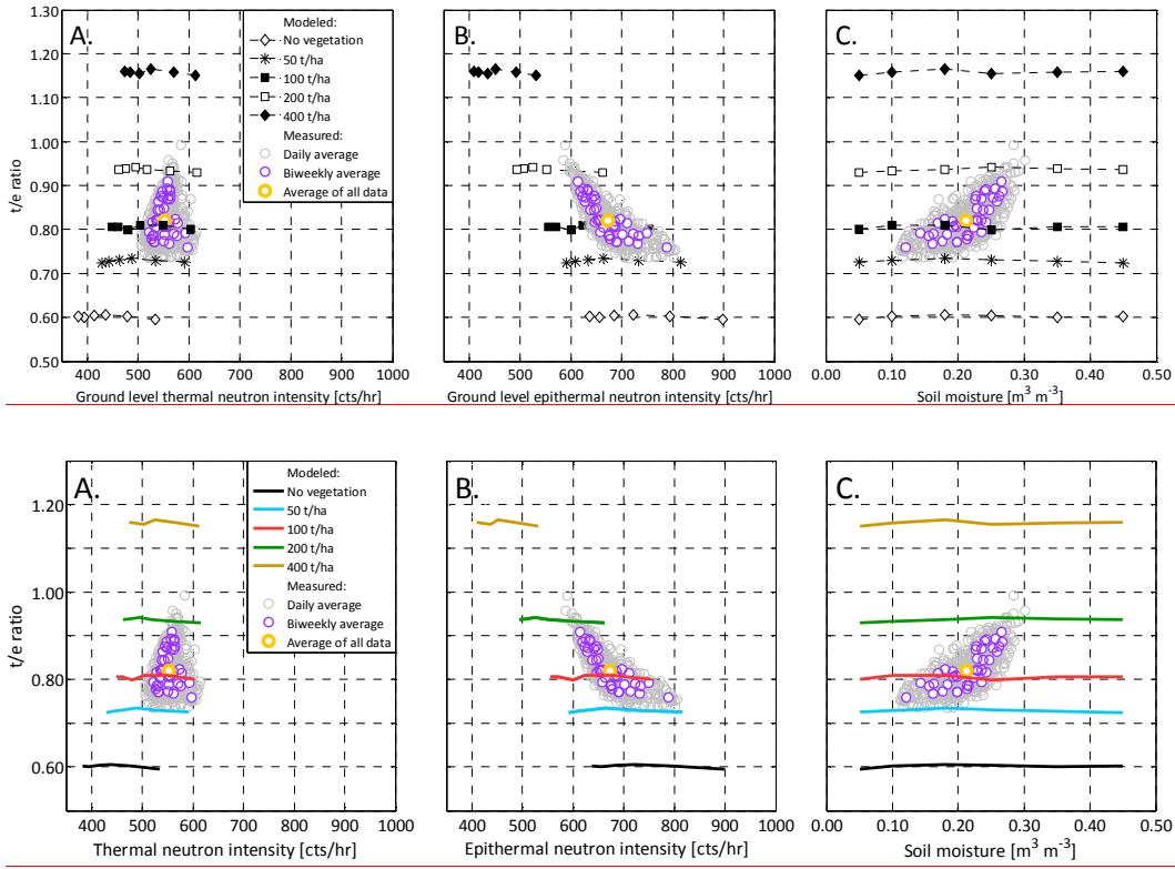
Figure 8 – Neutron intensities measured at Gludsted Plantation in the time period 2013-2015 and modeled using the Model Tree trunk, Foliage, Air . Ground level thermal-to-epithermal neutron intensity ratio plotted against measured and modeled: (A) ground level thermal neutron intensity, (B) ground level epithermal neutron intensity, and (C) volumetric soil moisture.
