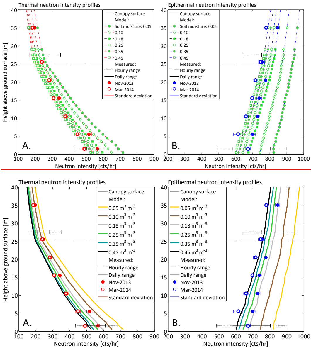
Figure 5 - Sensitivity to volumetric soil moisture, \text{in m}^3 \text{ m}^{-3} (using Model Foliage ). Measured and modeled (A) thermal and (B) epithermal neutron intensity profiles at Gludsted Plantation. Hourly and daily ranges of variation of thermal and epithermal neutron intensities at ground and canopy level for the period 2013–2015.
