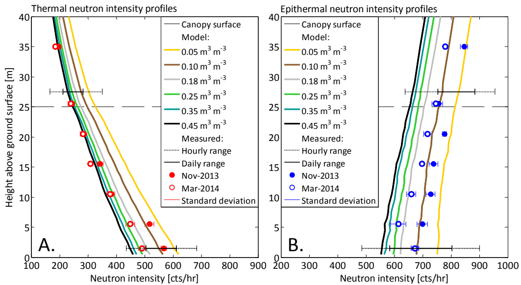
Figure 4 – Sensitivity to volumetric soil moisture, \text{m}^3 \text{m}^{-3} (using Model Tree trunk, Foliage, Air ). Measured and modeled (A) thermal and (B) epithermal neutron intensity profiles at Gludsted Plantation. Hourly and daily ranges of variation of thermal and epithermal neutron intensities at ground and canopy level for the period 2013–2015.
