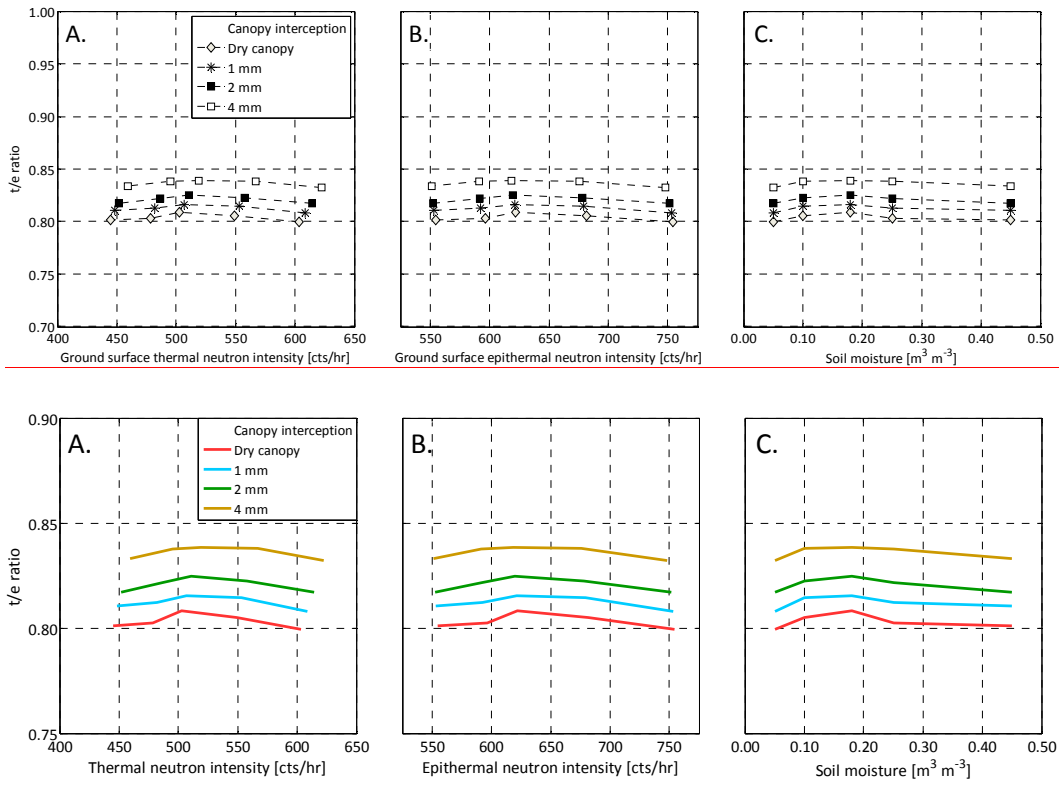
Figure 7 – Modeled ground level thermal-to-epithermal neutron intensity ratios using the Model Tree trunk, Foliage, Air for a dry forest canopy and canopy interception of 1 mm, 2 mm and 4 mm. plotted against modeled: (A) ground level thermal neutron intensity, (B) ground level epithermal neutron intensity, and (C) volumetric soil moisture.
