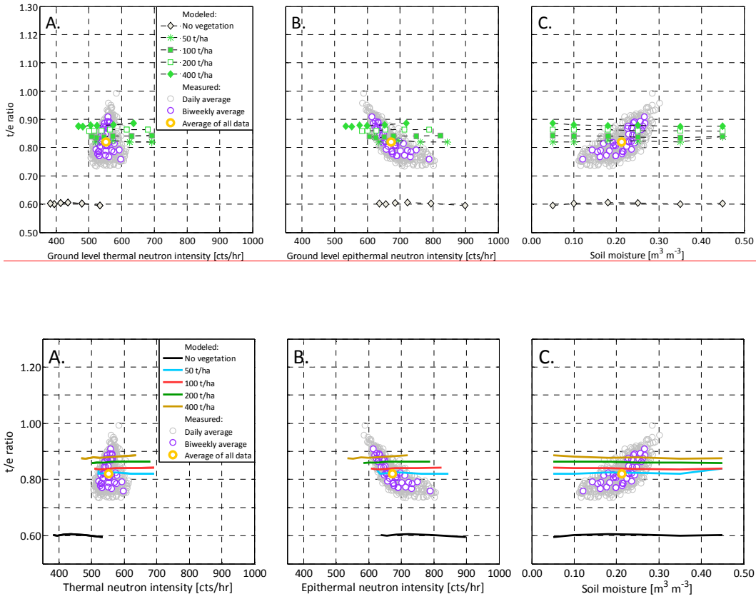
Figure 9 – Neutron intensities measured at Gludsted Plantation in the time period 2013-2015 and modeled using the Model Foliage . Ground level thermal-to-epithermal neutron intensity ratio plotted against measured and modeled: (A) ground level thermal neutron intensity, (B) ground level epithermal neutron intensity, and (C) volumetric soil moisture.
