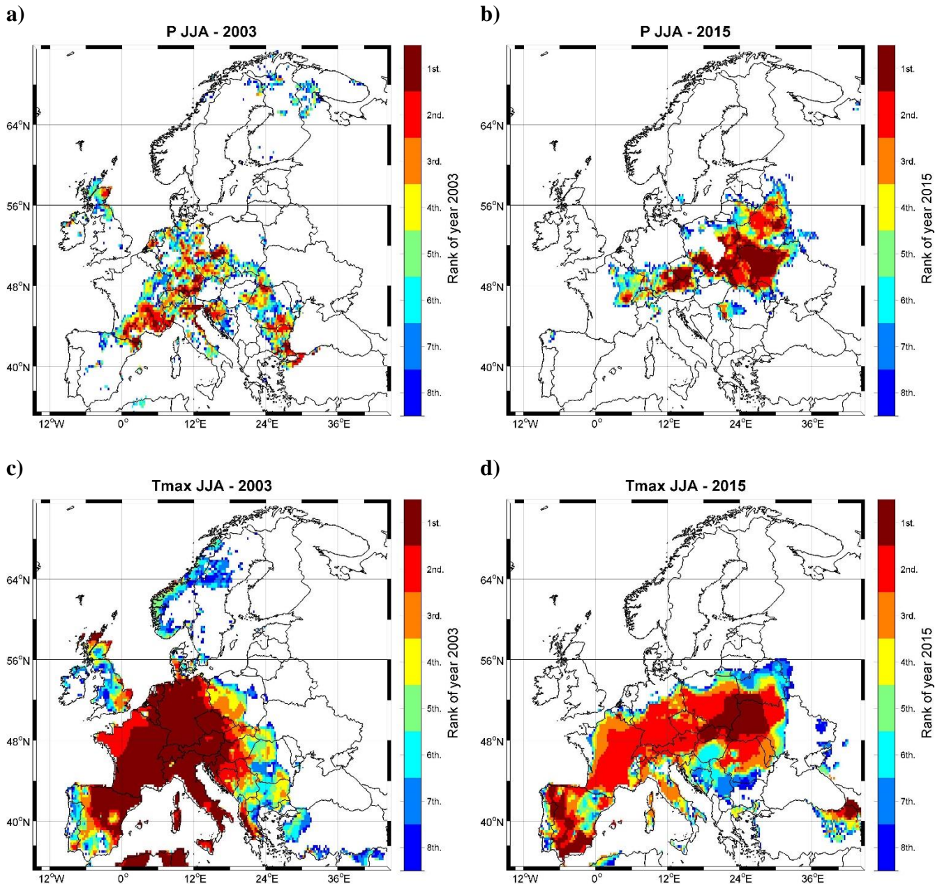
Figure 9. a) Top 8 ranking of 2003 summer P; b) Top 8 ranking of 2015 summer PP; c) Top 8 ranking of 2003 summer Tmax and d) Top 8 ranking of 2015 summer Tmax. In this figure, 1 means the driest (P) and warmest (Tmax) summer since 1950, 2 signifies the second driest, and all ranks greater than 8 are shown in white. Analyzed period: 1950 – 2015.
