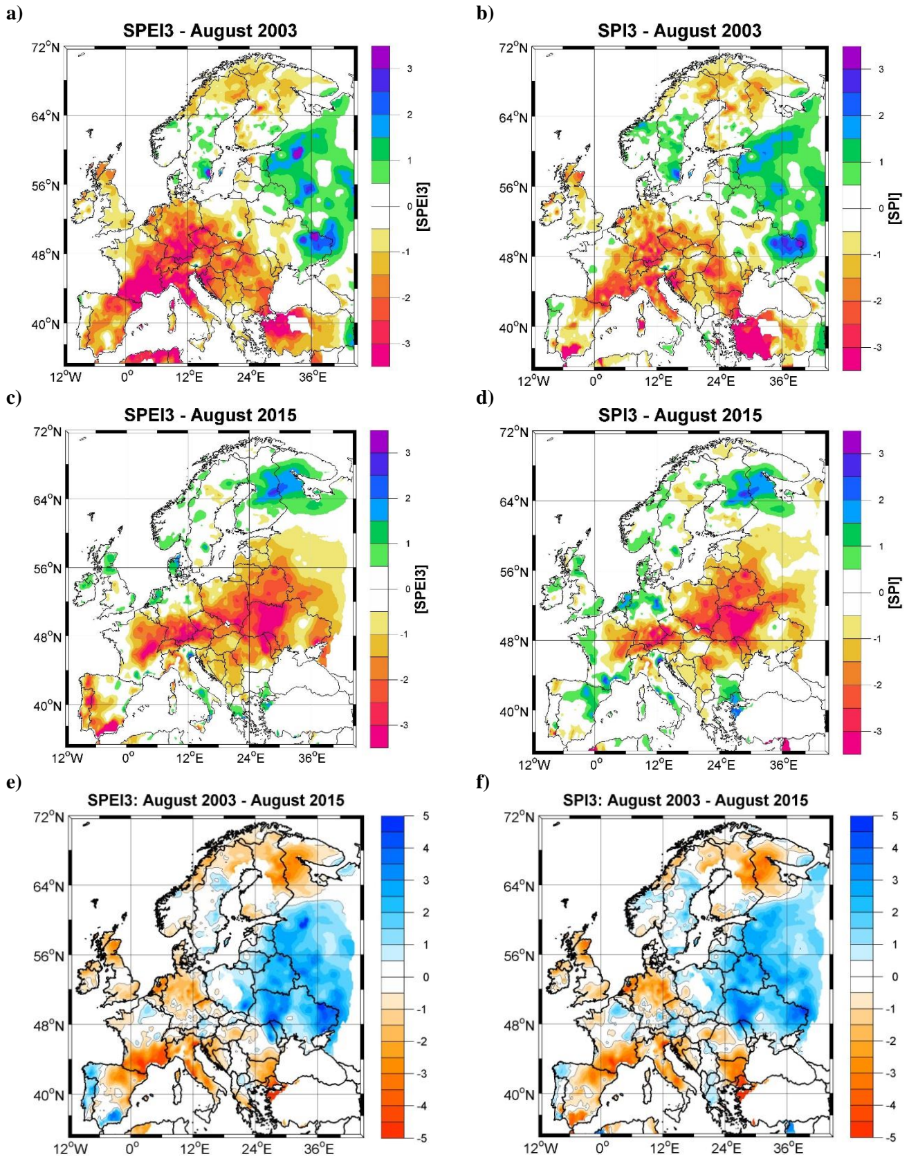
Figure 10. a) August 2003 SPEI3; b) as in a) but for SPI3; c) August 2015 SPEI3; d) as in a) but for SPI3; e) The difference between August 2003 SPEI3 and August 2015 SPEI3; f) as in e) but for SPI3.
