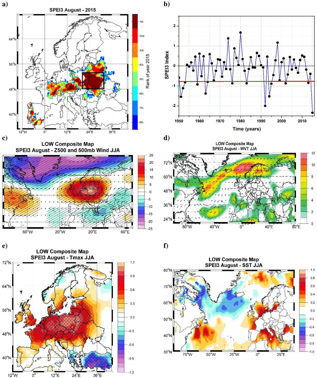
Figure 13. a) Top 8 ranking of 2015 August SPEI3; b) The time series of August SPEI3 index averaged over the black box in a); c) The Low (SPEI3 August index \leq 0.75 standard deviation)) composite map between the August SPEI3 index and the summer (JJA) Z500 and the wind vectors at 500mb; d) the same as c) but for the summer (JJA) WVT; e) the same as c) but for the summer (JJA) Tmax and f) the same as c) but for the summer (JJA) SST. Units: Z500(m), WVT ( \text{kg m s}^{-1} ), Tmax ( ^{\circ}\text{C} ) and SST ( ^{\circ}\text{C} ). The hatching highlights significant values at a confidence level of 95%. Analyzed period: 1950 – 2015.
