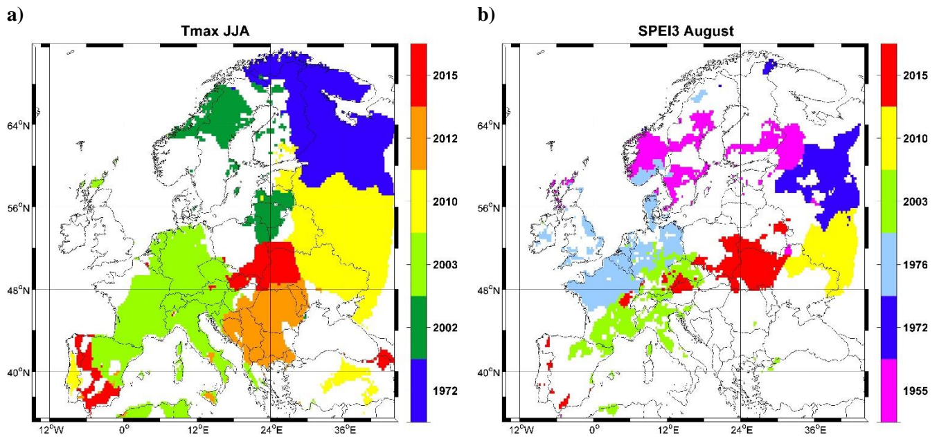
Figure 12. a) The spatial extent and the year of record of the warmest summers (Tmax JJA) over the last 66 years over Europe and b) same as in a) but for the driest years (SPEI3). Analyzed period: 1950 – 2015.
