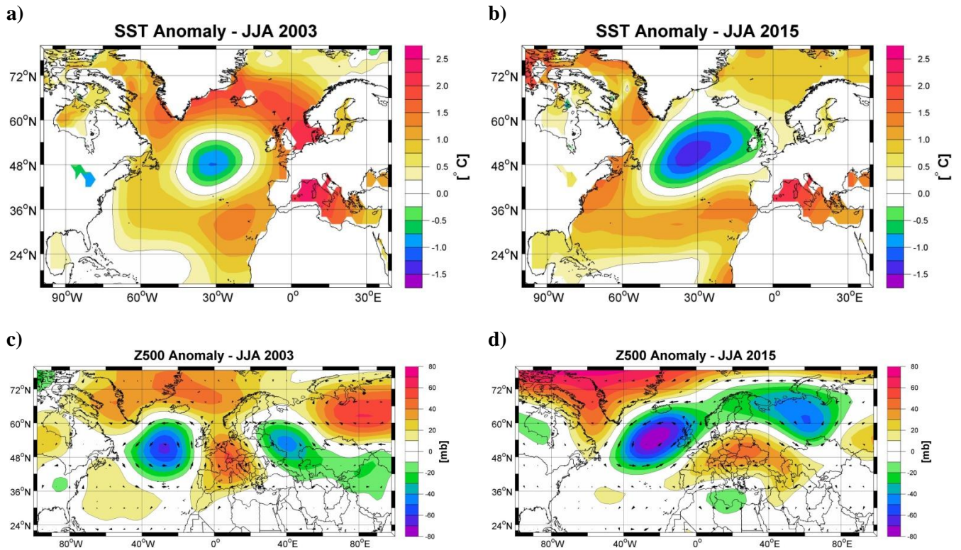
Figure 11. a) Summer 2003 SST anomalies; b) as in a) but for summer 2015; c) Summer 2003 Z500 anomalies and d) as in c) but for summer 2015. The anomalies are computed relative to the period 1971 – 2000.
