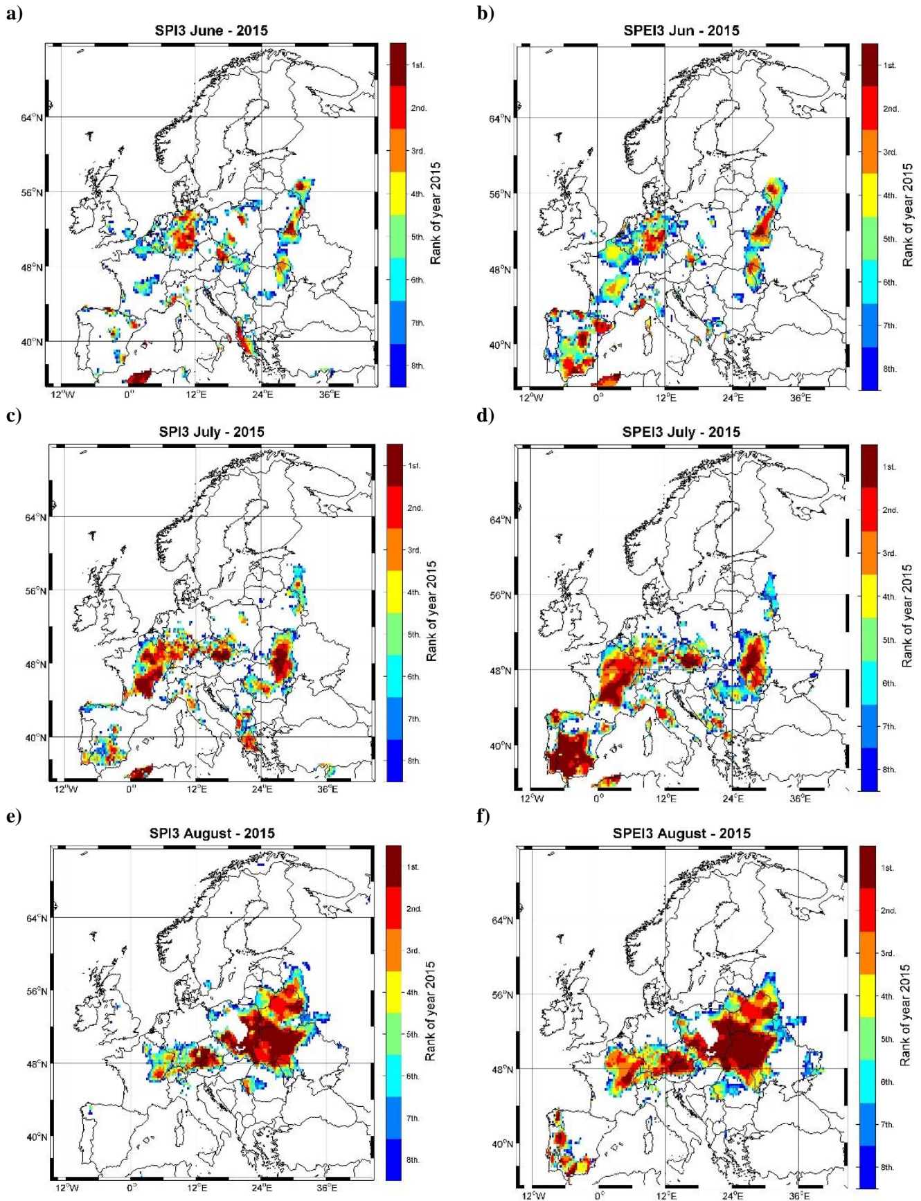
Figure 3. Top 8 ranking of 2015 monthly SPI3 (left column) and 2015 SPEI3 (right column): a) June SPI3; b) June SPEI3; c) July SPI3; d) July SPEI3; e) August SPI3 and f) August SPEI3. In this figure, 1 means the driest month since 1950, 2 signifies the second driest, and all ranks greater than 8 are shown in white. Analyzed period: 1950 – 2015.
