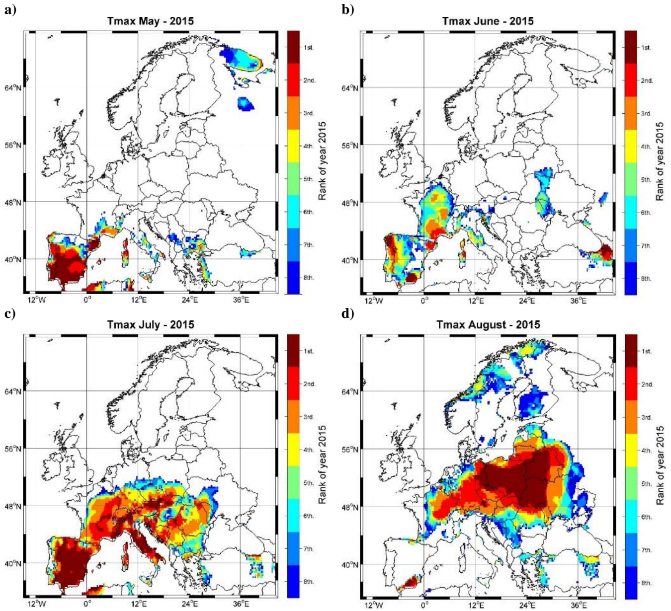
Figure 2. Top 8 ranking of 2015 monthly Tmax: a) May Tmax; b) June Tmax; c) July Tmax and d) August Tmax. In this figure, 1 means the warmest (TT) month since 1950, 2 signifies the second warmest, and all ranks greater than 8 are shown in white. Analyzed period: 1950 – 2015.
