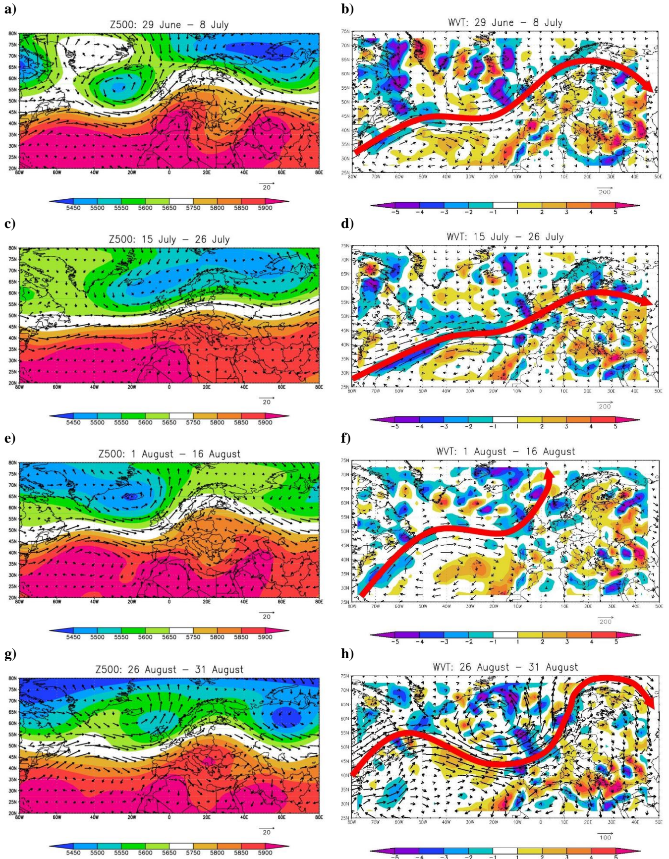
Figure 7. Mean daily Z500 (left column) and WVT (right column) averaged over: a) and b) 29 June – 8 July; c) and d) 15 July – 26 July; e) and f) 1 August – 16 August and g) and h) 26 August – 31 August. Units: Z500 (mb)
