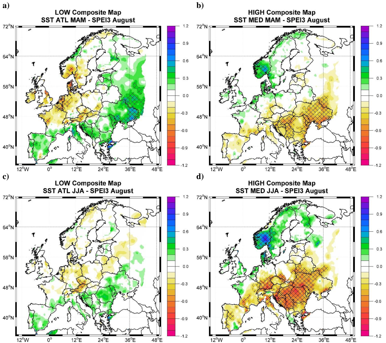
Figure 15. a) The Low (SST cold Index \leq 0.75 standard deviation) composite map between the spring (MAM) Atlantic SST cold index (defined as the MAM averaged SST over the black box in Figure 9a) and the August SPEI3 field; b) The High (SST Warm Index \geq 0.75 standard deviation) composite map between the spring (MAM) Mediterranean SST Warm index (defined as the MAM averaged SST over the black box in Figure 9b) and the August SPEI3 field c) same as a) but for summer (JJA) Atlantic SST and d) same as in b) but for the summer (JJA) Mediterranean SST. The hatching highlights significant values at a confidence level of 95%. Analyzed period: 1950 – 2015.
