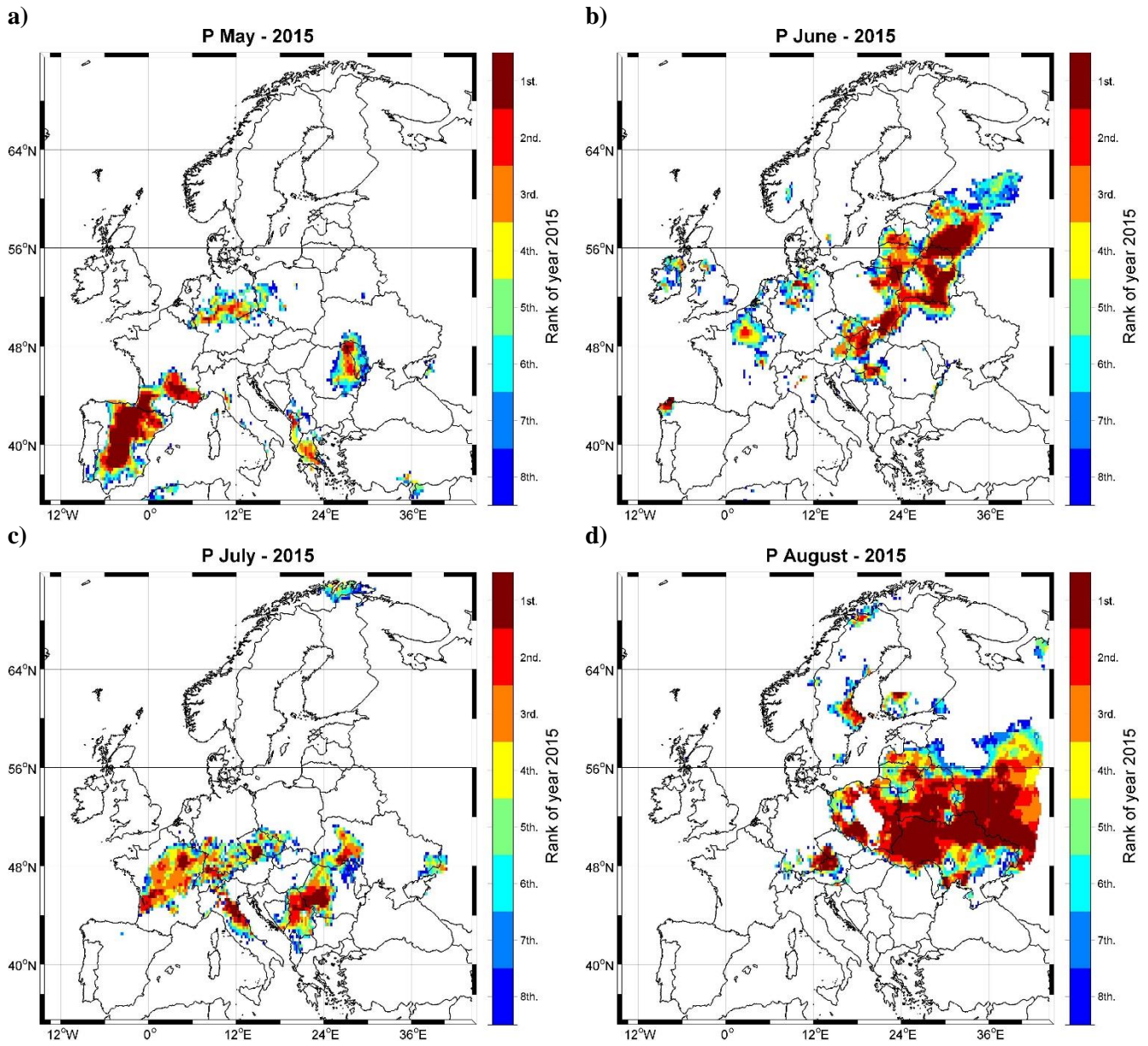
Figure 1. Top 8 ranking of 2015 monthly lowest P: a) May P; b) June P; c) July P and d) August P. In this figure, 1 means the driest (P) month since 1950, 2 signifies the second driest, and all ranks greater than 8 are shown in white. Analyzed period: 1950 – 2015.
