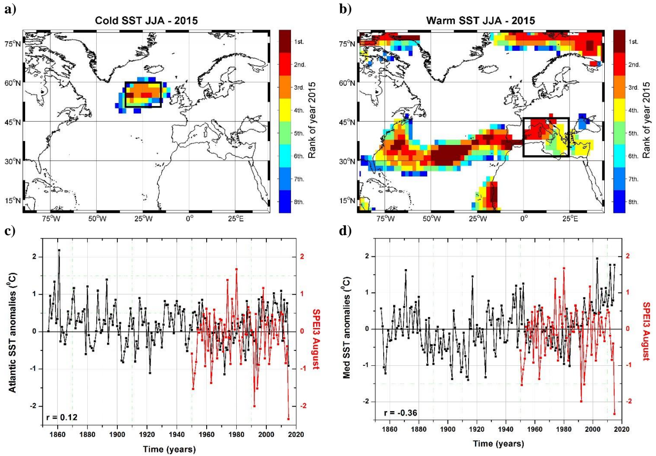
Figure 14. a) Top 8 ranking of 2015 summer (JJA) cold SST; b) Top 8 ranking of 2015 summer (JJA) warm SST; c) The time series of JJA cold SST index averaged over the black box in a) (black line) and the time series of August SPEI3 index averaged over the black box in Figure 7a (red line); d) The time series of JJA warm SST index averaged over the black box in b) and the time series of August SPEI3 index averaged over the black box in Figure 7a (red line). The Atlantic SST index and the Med SST index are based on the ERSSTv4b dataset [Liu et al., 2014]. Analyzed period: 1854 – 2015.
