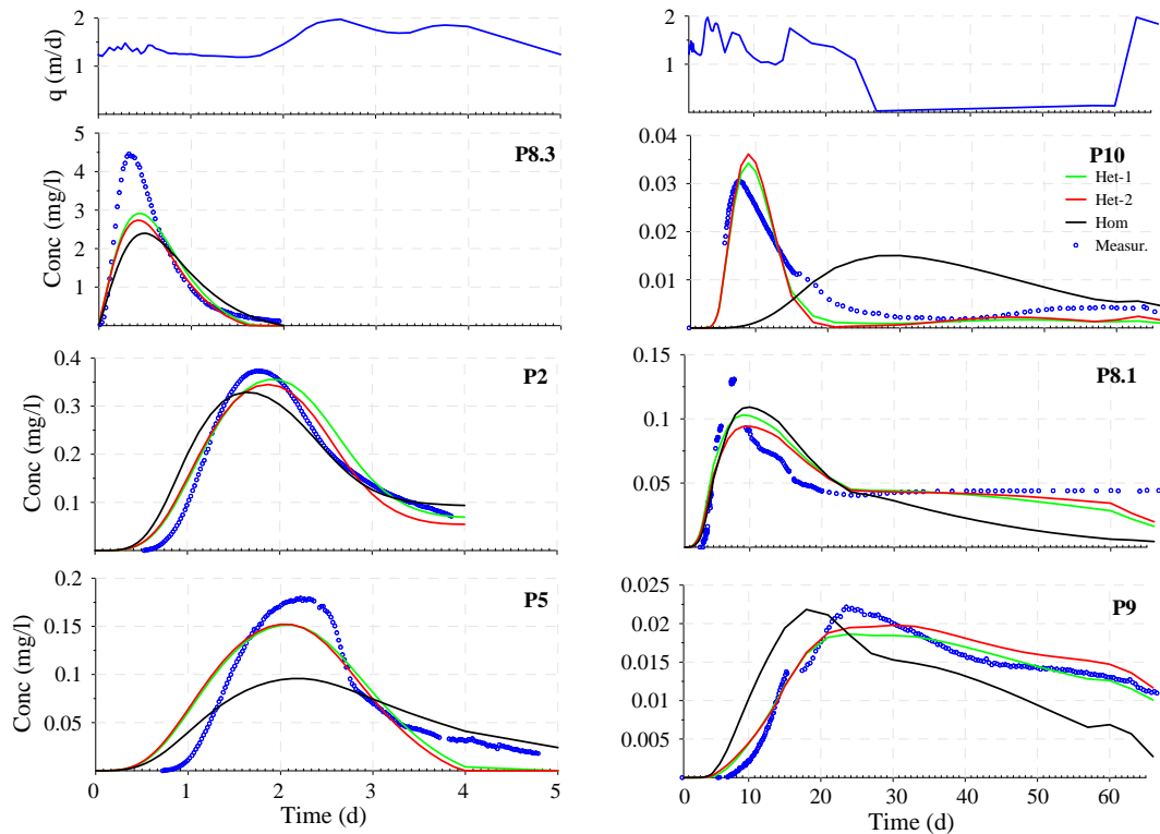
Figure 3. Top row, inflow rate to the infiltration basin and lower three rows measured (blue circles) and calculated breakthrough curves from the piezometers monitoring of the amino-G acid concentration (mg/l) vs. time (d) using the estimated set of parameters of Het-1 (green line), Het-2 (red line), and Hom (black line). The left row displays only the first five days of the experiment. Note that the vertical scale is different for each monitoring point.
