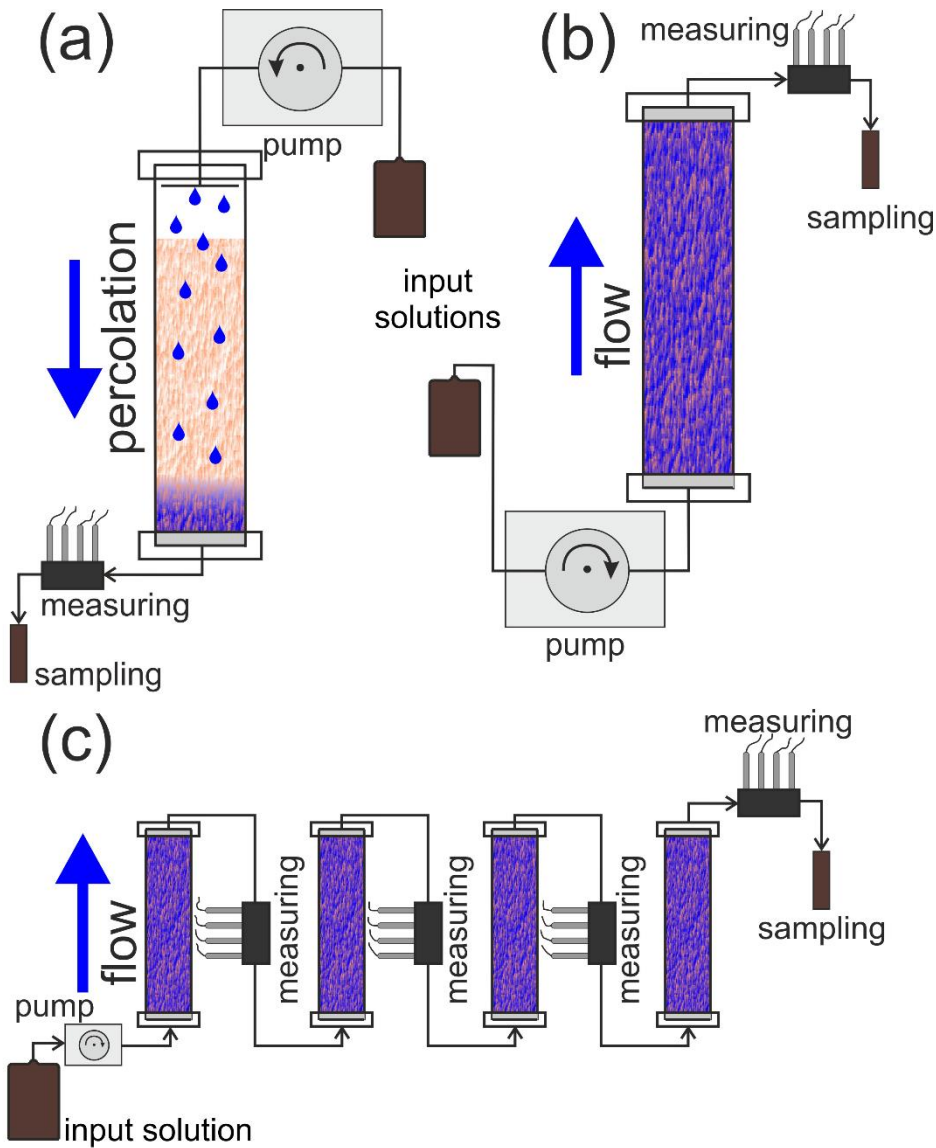
Figure 2: Schema of common setups used in columns experiments: (a) unsaturated / leaching experiments (e.g. Siemens et al., 2010); a fluctuating water table is established in some experimental setups (e.g. Sinke et al., 1998), (b) saturated / groundwater flow experiments (e.g. Scheytt et al., 2004), (c) saturated columns connected in series in order to measure the evolution of hydrochemical parameters (such as the oxidation-reduction potential) along the flow path (e.g. Nay et al., 1999).
