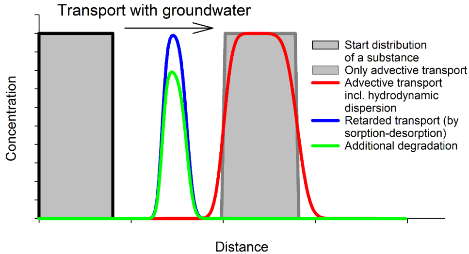
Figure 1: Schematic representation of solute transport in groundwater, taking into account the main transport processes of advection, hydrodynamic dispersion, retardation, and degradation. BTCs were modelled using the CXTFIT code (Toride et al., 1999). Model was setup as Deterministic equilibrium CDE with flux-averaged concentration and dimensionless parameters.
