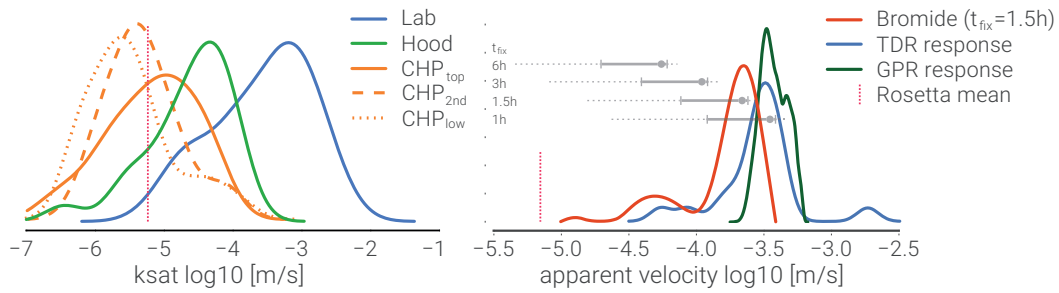
Figure 9. Saturated hydraulic conductivity and apparent vertical flow velocity kernel density estimates. Left panel: Point scale measurement results (Lab: Ksat apparatus, Hood: Hood Tension-Infiltrometer, CHP: Constant Head Permeameter in different depth levels); Right panel: Results from plot scale irrigation experiments. Vertical gray lines are box plots of velocity distribution based on different t_{fix} estimates for Bromide. Rosetta (Schaap et al., 2001) reference based on mean values of ring samples (15.7, 47.9, 36.4 % sand, silt, clay and BD 1.1 \text{g cm}^{-3} )
