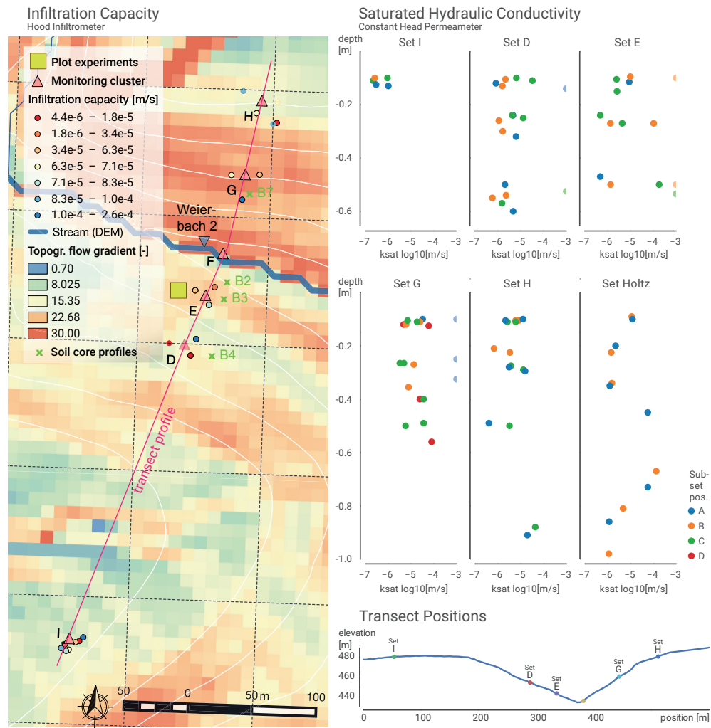
Figure 13. Hydrological exploration results. Left: Infiltration capacity (values color coded) measured with hood infiltrometer. Basemap with topographic flow gradient G = \arctan(\partial z_{rel}/\partial d_{rel}) , topography contour lines and positions of hydro-meteorological monitoring clusters. Right top: Saturated hydraulic conductivity measured with a constant head permeameter. Individual profile position in the respective nested set color coded (2 measurement holes with dist=1 m). Values exceeding the device capacity set to 10^{-3} \text{ m s}^{-1} . Right bottom: Elevation profile of transect as characteristic landscape feature in the sub-basin.
