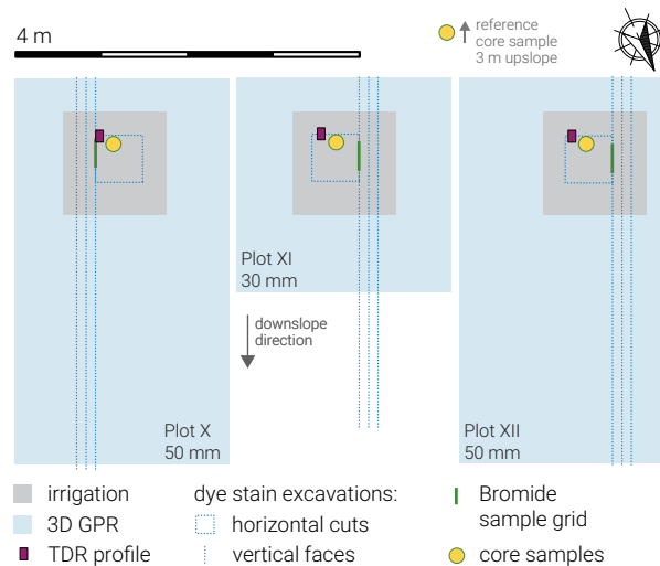
Figure 2. Plan view layout of the plot scale irrigation experiments. Three irrigation plots (1 m 2 , gray squares) are monitored by 3D time-lapse GPR (blue rectangles) and TDR (soil moisture tube probe, red box). The plots are sampled for tracer recovery by percussion drilled core samples (yellow dot) and in a grid on the last of three vertical faces (dashed blue line). Moreover, dye stains are excavated at horizontal cuts in the center of the irrigation area (dashed blue square). A pre-irrigation reference for pore water stable isotope composition is sampled as fourth core 3 m upslope.
