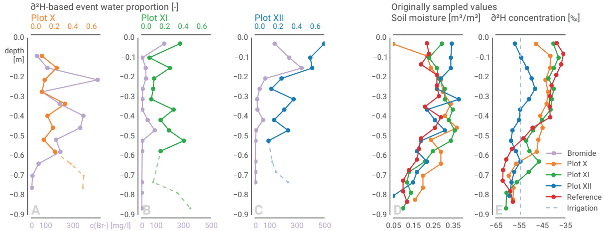
Figure 15. Plot scale irrigation experiments. Proportion of event water derived from deviations in concentration of Deuterium and Bromide in soil water of sampled cores to reference (A-C). Absolute measured soil water content (D). Deuterium concentration in samples and signature of irrigation water (E). Note that the \delta^2\text{H} concentration profiles and the signature of the irrigation water show low deviation and even coincide in 0.5 m depth. Thus the interpretation needs precaution, especially below that level (dashed lines A-C).
