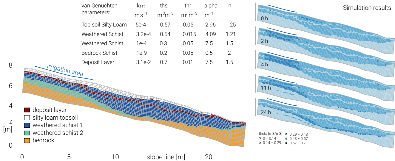
Figure 14. CATFLOW model reference of hillslope experiment. Left panel: Table of used soil definitions and hypothetical hillslope setup. Right panel: Simulated soil moisture with 30\text{ mm h}^{-1} irrigation for 4h.
