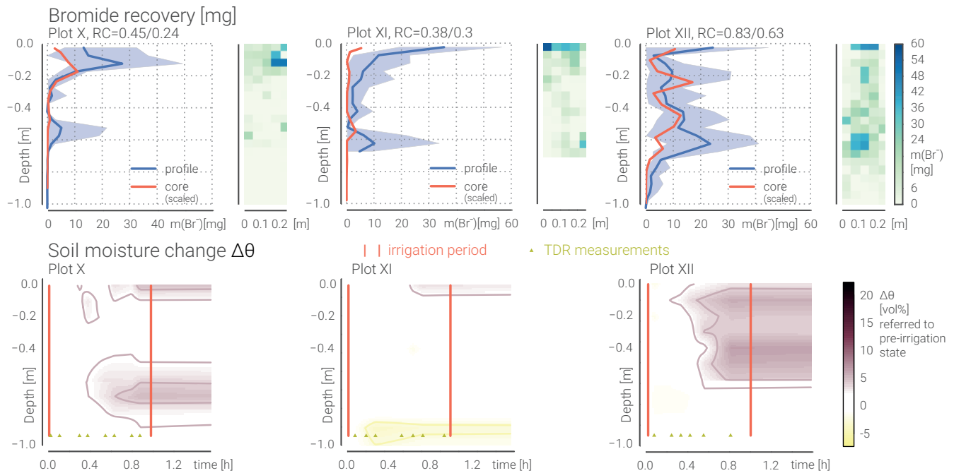
Figure 7. Results from plot scale irrigation experiments with 50mm, 30mm and 50mm spray irrigation for 1 h. Top: Recovered Bromide mass profiles and grids (5x5cm). Blue line as mean and shaded area between min/max for each depth of the sampling grid. Orange line is mass recovered in drilled profile samples (scaled to same volume reference). Recovery coefficient (RC) calculated for the profile samples (first value) and the profile and core samples (second value). Bottom: Observed soil moisture change referenced to the first measurement shortly before onset of the irrigation. Individual measurement times marked with triangles.
