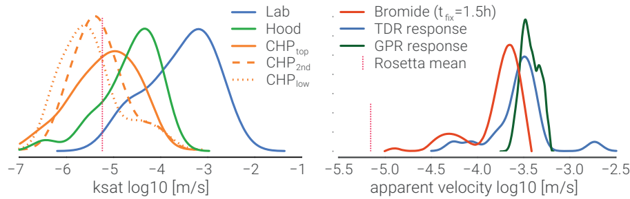
Figure 9. Saturated hydraulic conductivity and apparent vertical flow velocity kernel density estimates. Left panel: Point scale measurement results (Lab: Ksat apparatus, Hood: Hood Tension-Infiltrometer, CHP: Constant Head Permeameter in different depth levels); Right panel: Results from plot scale irrigation experiments. Rosetta (Schaap et al., 2001) reference based on mean values of ring samples (15.7, 47.9, 36.4 % sand, silt, clay and BD 1.1 \text{ g cm}^{-3} )
