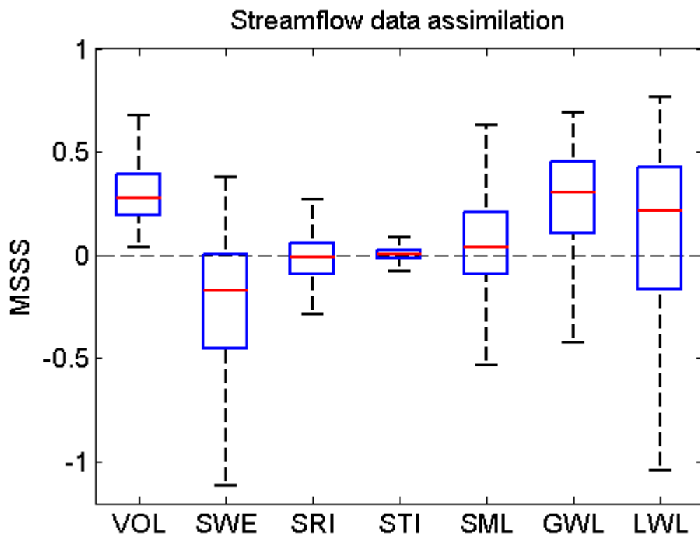
Figure 4: Box plot of the Mean Square Skill Score for each variable when assimilating streamflow at the outlet. The open loop is used as a reference. Outliers are not shown for visibility purposes.
