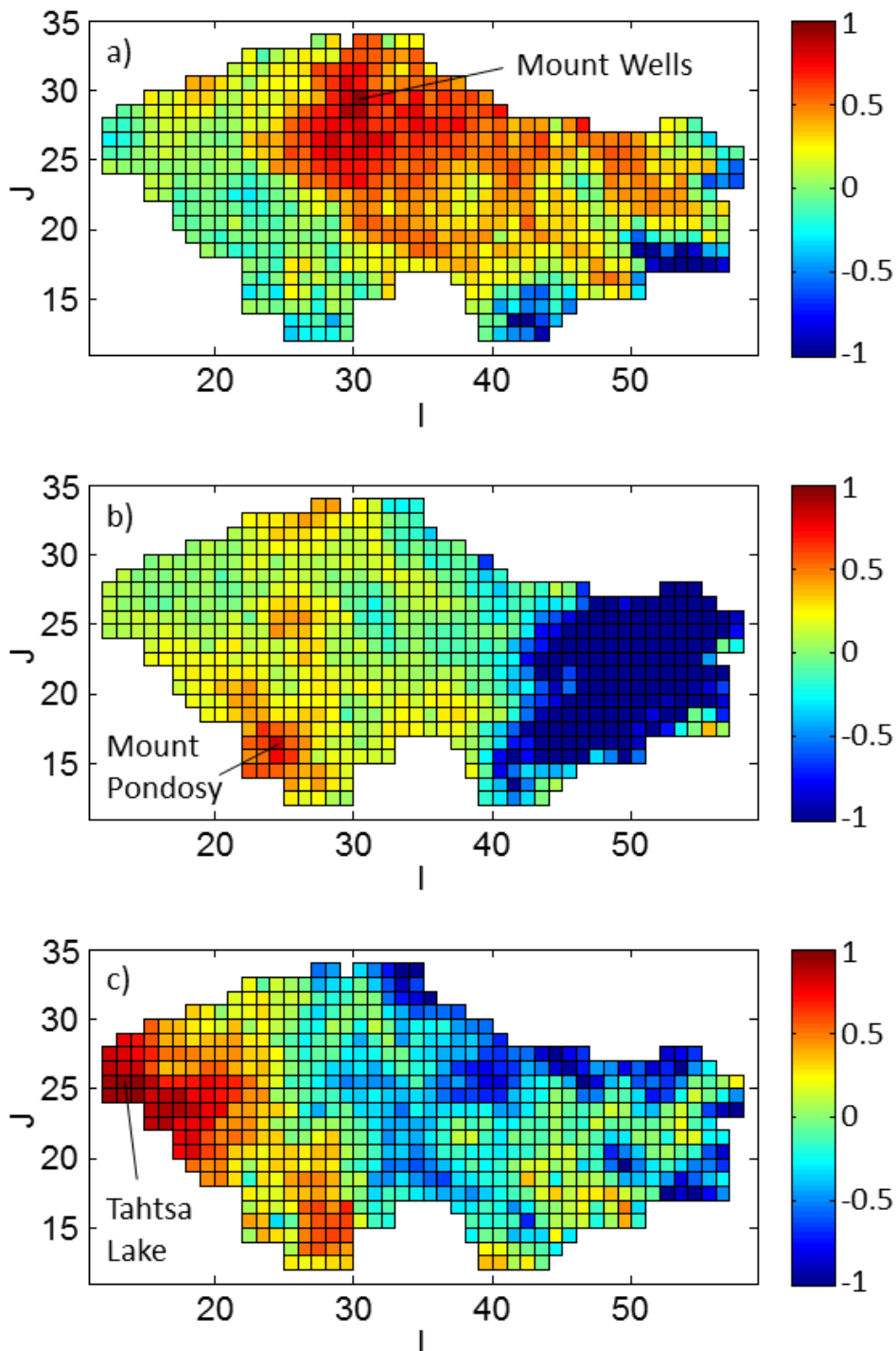
Figure 5: Distribution of the Mean Square Skill Score of SWE over the watershed when assimilating SWE located at a) Mount Wells, b) Mount Pondosy and c) Tahtsa Lake. The open loop is used as a reference. Values below -1 are cut off from the legend.
