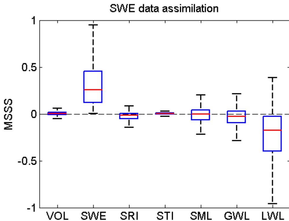
Figure 6: Box plot of the Mean Square Skill Score for each variable when assimilating SWE from all three snow pillow locations. The open loop is used as a reference. Outliers are not shown for visibility purposes.
