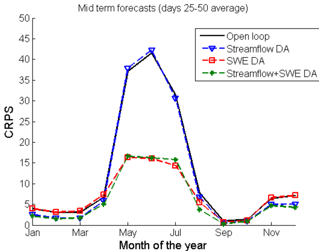
Figure 12: Continuous Rank Probability Score for mid-term forecasts (average of forecast horizons 25 through 50 days) of various data assimilation scenarios as a function of the month of the year.
