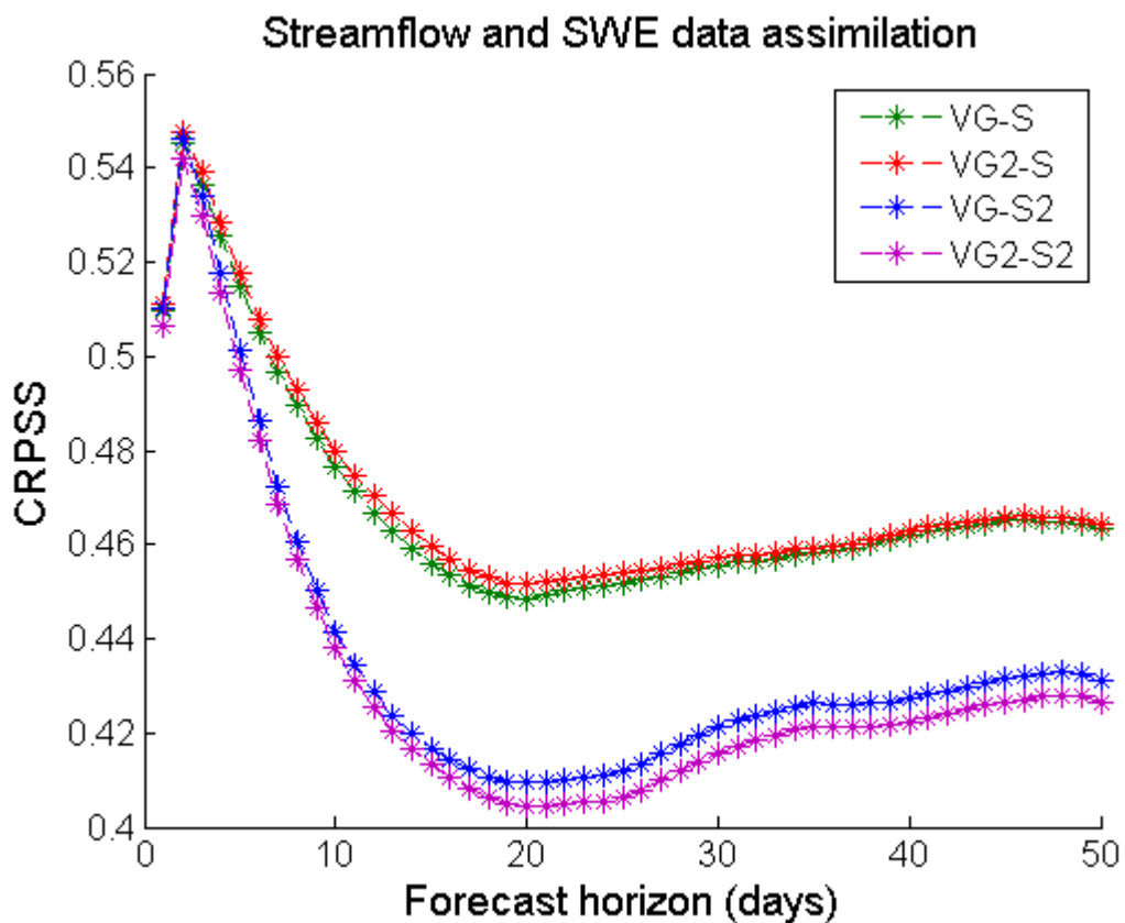
Figure 10: Continuous Rank Probability Skill Score of the streamflow ensemble when assimilating streamflow at the outlet and SWE from all three snow pillow locations. The open loop is used as a reference. The forecast horizon varies from 1 to 50 days. Lack of parentheses indicates that the variable is affected by both types of observations.
