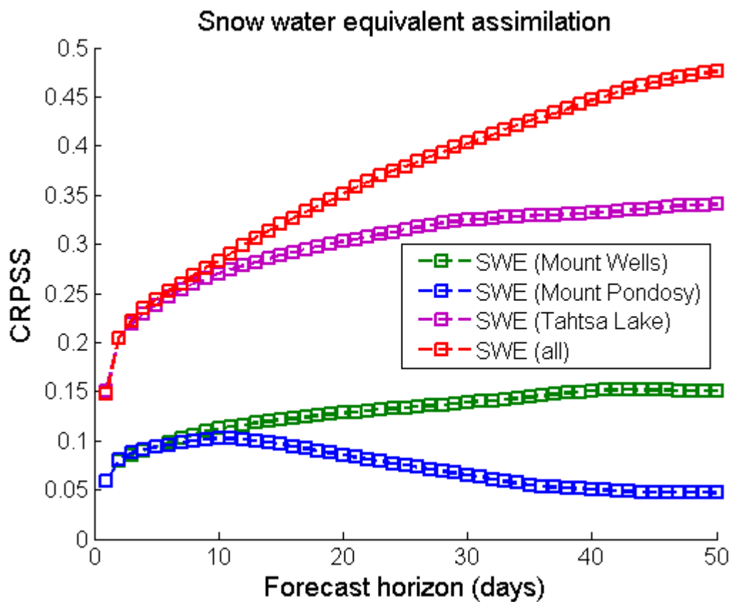
Figure 9: Continuous Rank Probability Skill Score of the streamflow ensemble when assimilating SWE from all three snow pillow locations. The open loop is used as a reference. The forecast horizon varies from 1 to 50 days.
