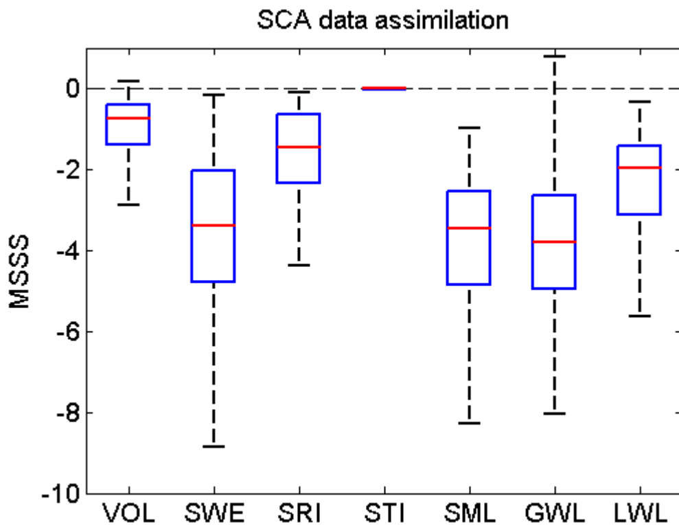
Figure 7: Box plot of the Mean Square Skill Score for each variable when assimilating basin-wide snow cover area. The open loop is used as a reference. Outliers are not shown for visibility purposes.
