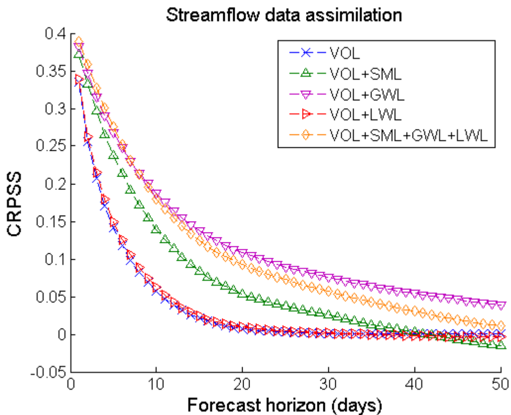
Figure 8: Continuous Rank Probability Skill Score of the streamflow ensemble when assimilating streamflow at the outlet. The open loop is used as a reference. The forecast horizon varies from 1 to 50 days.
