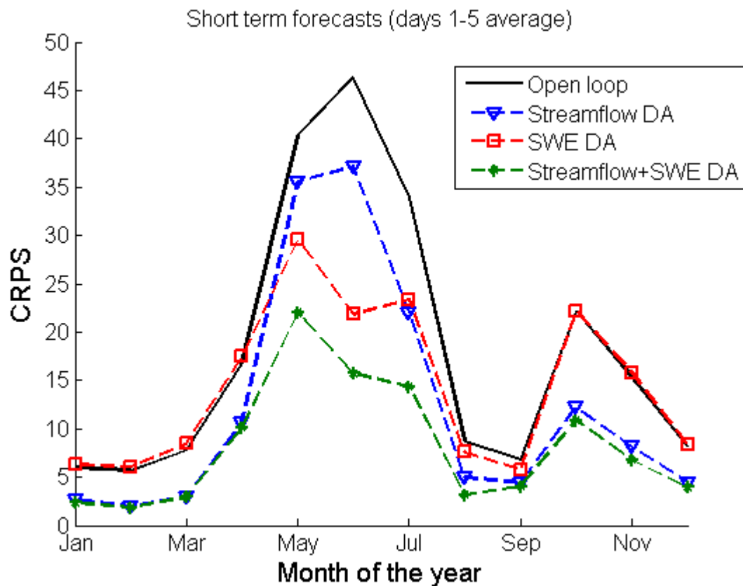
Figure 11: Continuous Rank Probability Score for short-term forecasts (average of forecast horizons 1 through 5 days) of various data assimilation scenarios as a function of the month of the year.
