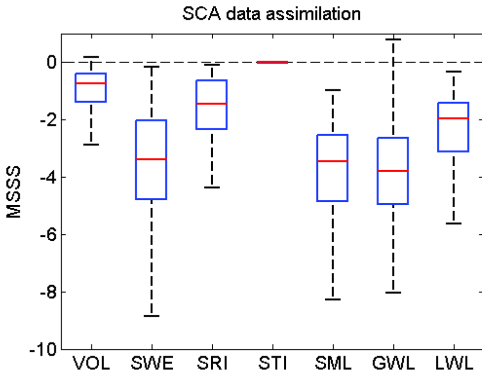
Figure 8: Box plot of the Mean Square Skill Score for each variable when assimilating basin-wide snow cover area. The open loop is used as a reference. Outliers are not shown for visibility purposes.
