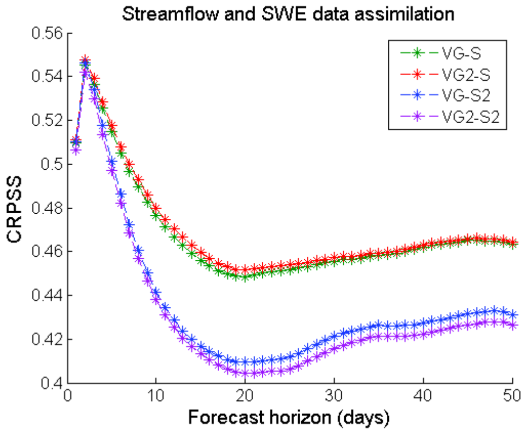
Figure 11: Continuous Rank Probability Skill Score of the streamflow ensemble when assimilating streamflow at the outlet and SWE from all three snow pillow locations. The open loop is used as a reference. The forecast horizon varies from 1 to 50 days. Lack of parentheses indicates that the variable is affected by both types of observations.
