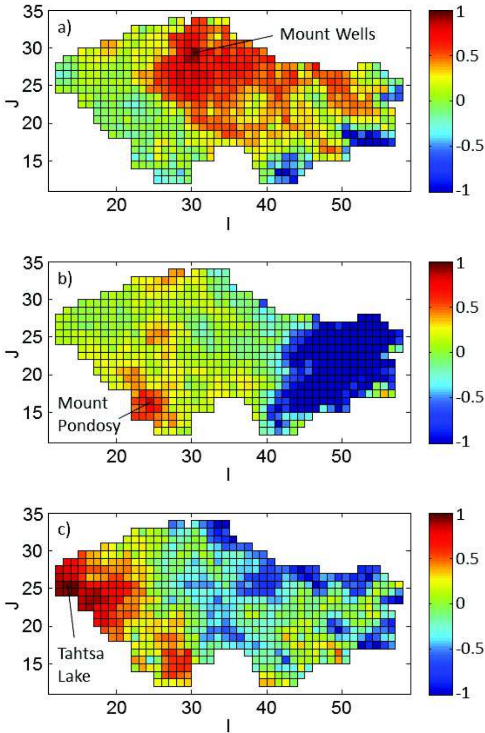
Figure 6: Distribution of the Mean Square Skill Score of SWE over the watershed when assimilating SWE located at a) Mount Wells, b) Mount Pondosy and c) Tahtsa Lake. The open loop is used as a reference. Values below -1 are cut off from the legend.
