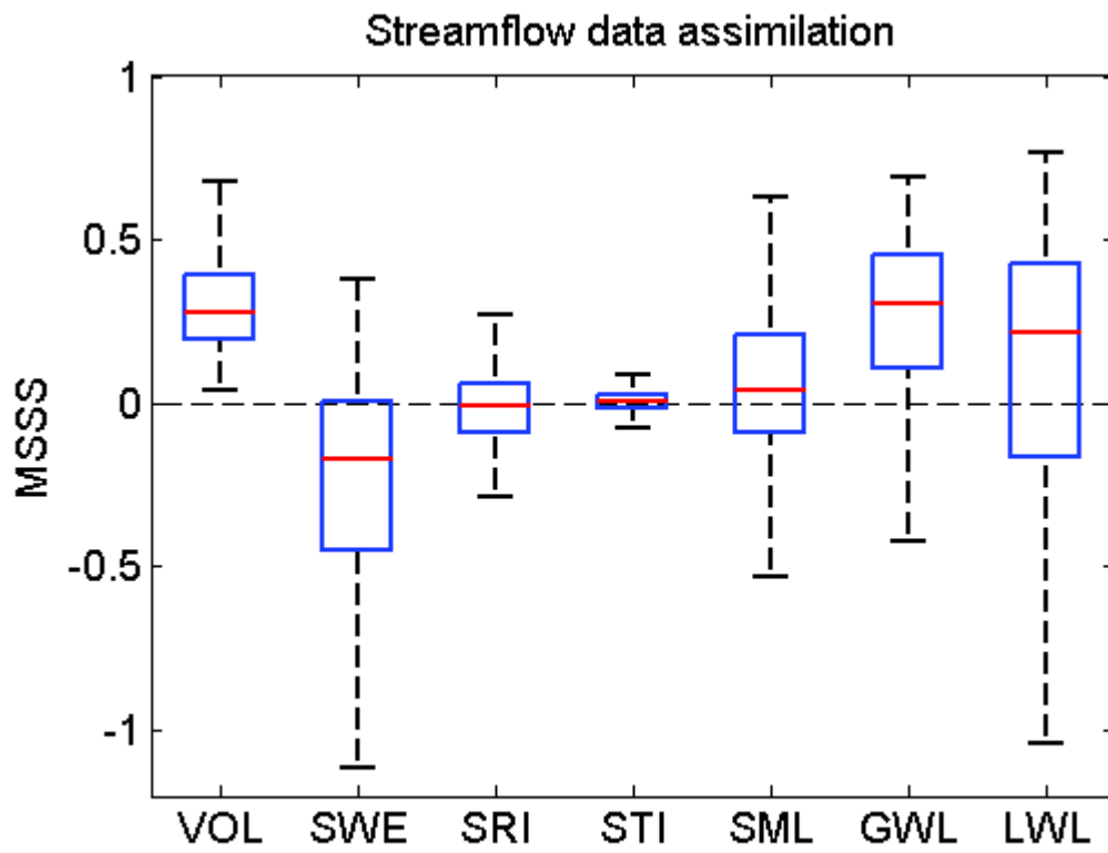
Figure 5: Box plot of the Mean Square Skill Score for each variable when assimilating streamflow at the outlet. The open loop is used as a reference. Outliers are not shown for visibility purposes.
