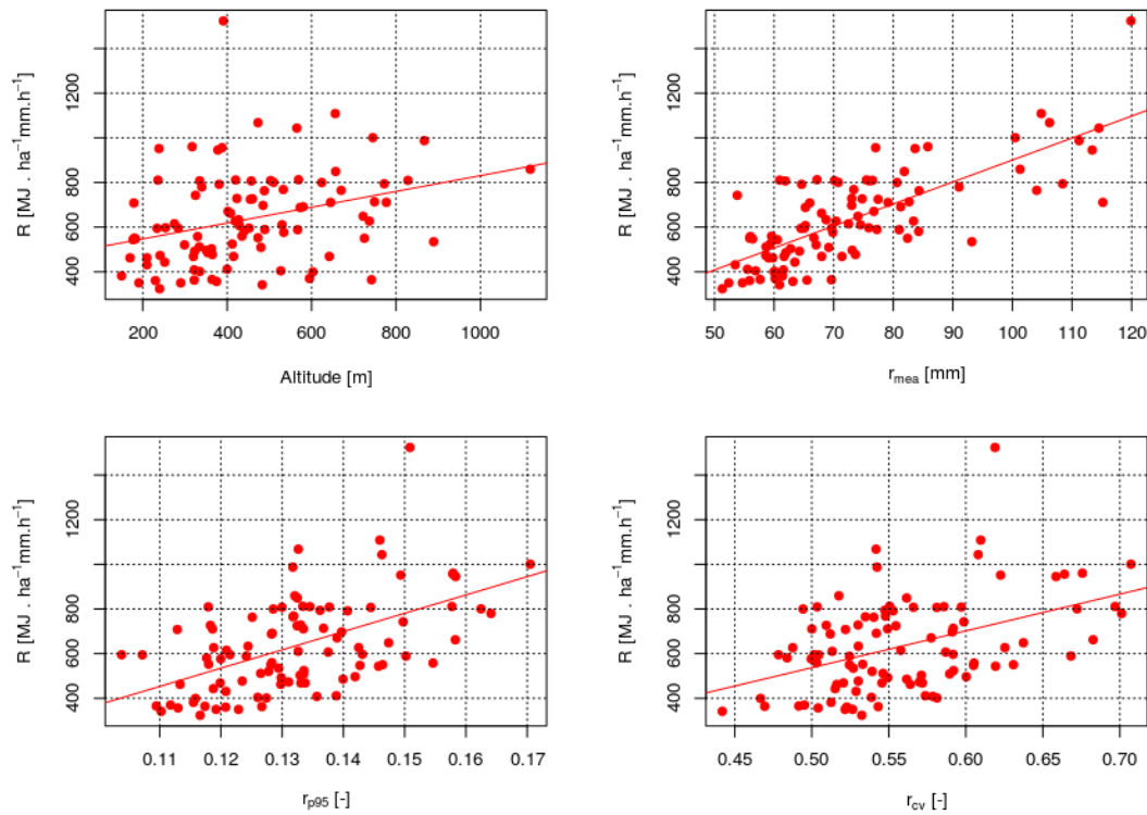
Fig. 3. Scatter plots for Rfactor and selected covariates.
