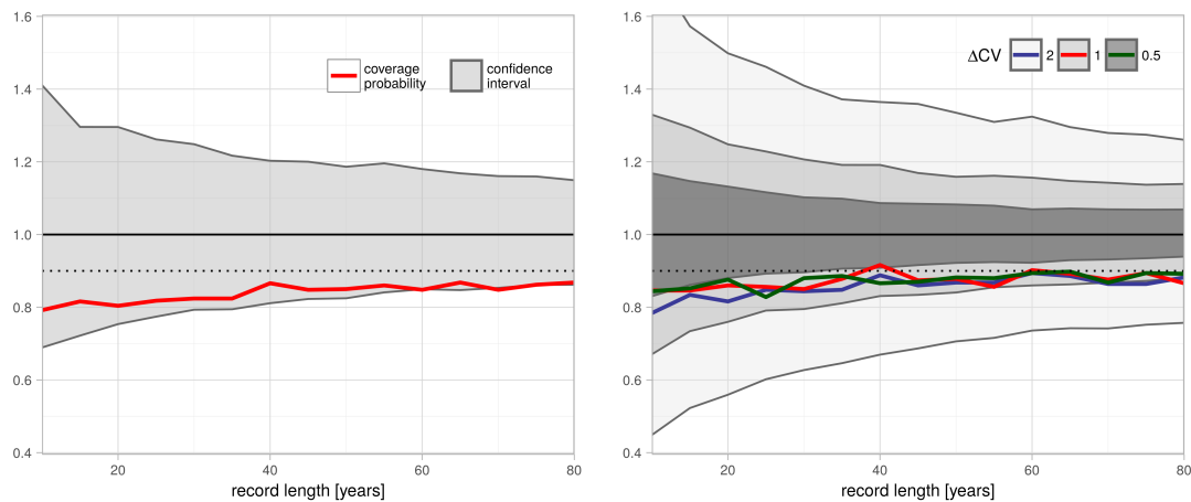
Fig. 1. The average confidence intervals (relative to the long-term mean R-factor, 669 MJ h^{-1} mm h^{-1} ; gray area) and the coverage probability (thick lines) for different record lengths based on the
