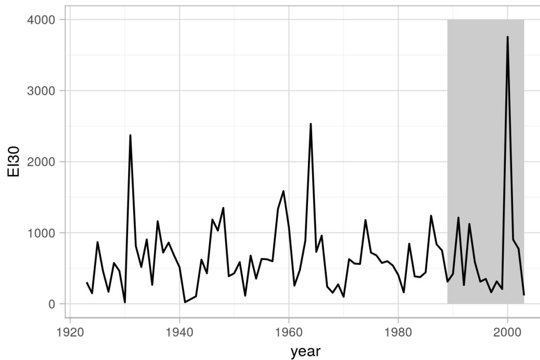
Fig. 2. Annual erosivity index (EI30) for station C2TREB01
