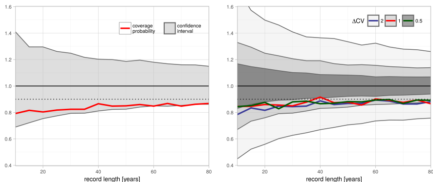
Figure 6. The average confidence intervals (relative to the long-term mean R-factor, 669 \text{ MJ ha}^{-1} \text{ mm h}^{-1} ; gray area) and the coverage probability ( red linethick lines ) for different record lengths based on the station C2TREB01 ( ← Třeboň (left) and simulated data (right) ). The dotted line corresponds to the coverage probability of 90%.
