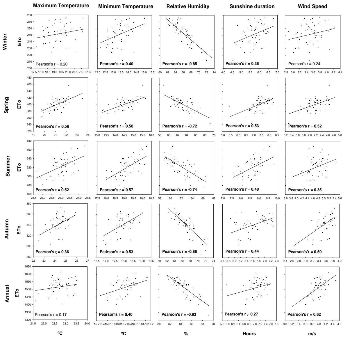
Figure 7. Relationship between the regional annual and seasonal ETo and the regional series of the different meteorological variables. Pearson's coefficients are included in each plot. In bold the coefficients statistically significant at the 0.95 confidence level
