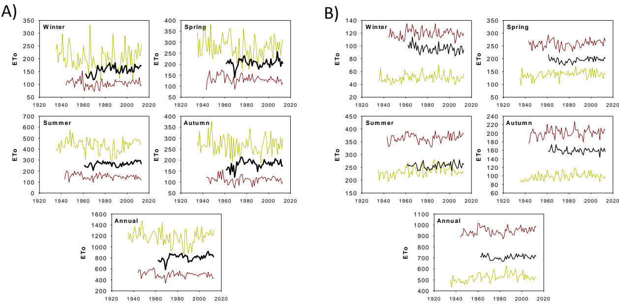
729 Figure 6: Evolution of seasonal and annual aerodynamic (A) and radiative (B) components of the 730 ET0 in the two meteorological stations with longest records (Izaña, green and Santa Cruz de 731 Tenerife, brown) and the average of the eight stations (black lines) from 1961 to 2013
