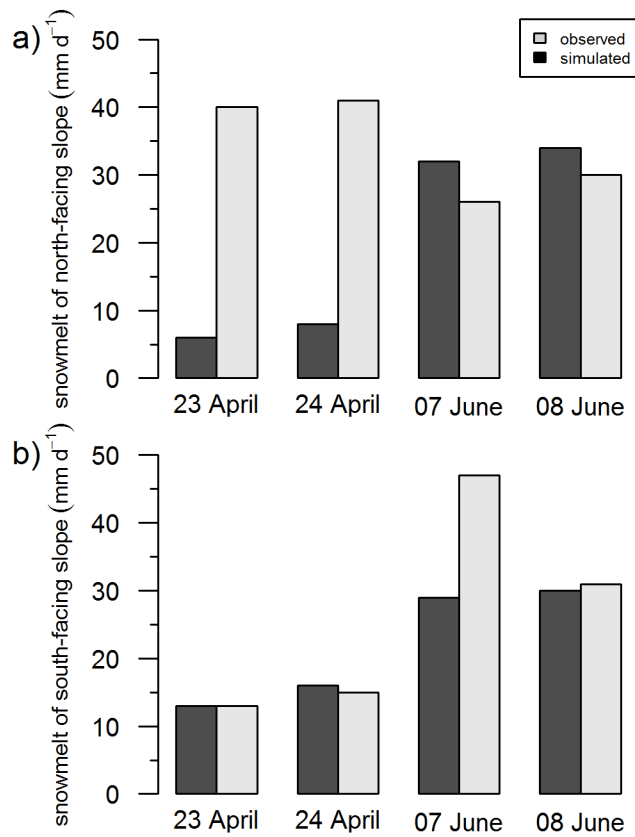
Figure 10: Differences between the observed (plot scale) and simulated (catchment scale) daily snowmelt on (a) the north-facing and (b) the south-facing slope for the early melt (23/24 April) and peak melt (07/08 June).
