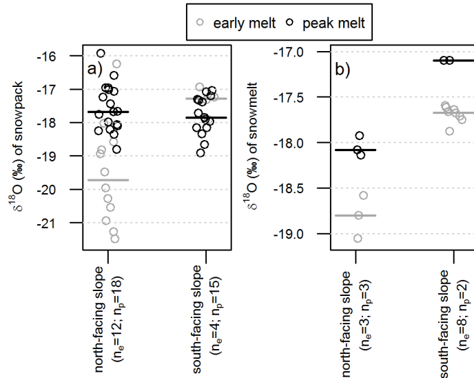
Figure 6: Jittered dot plots for \delta^{18}\text{O} of (a) snowpack and (b) snowmelt of north- and south-facing slopes. Grey circles indicate early melt samples and black circles are for peak melt samples. The grey and black line indicates the median of the early and peak melt data, respectively. N_e is the number of early melt samples and n_p is the number of peak melt samples.
