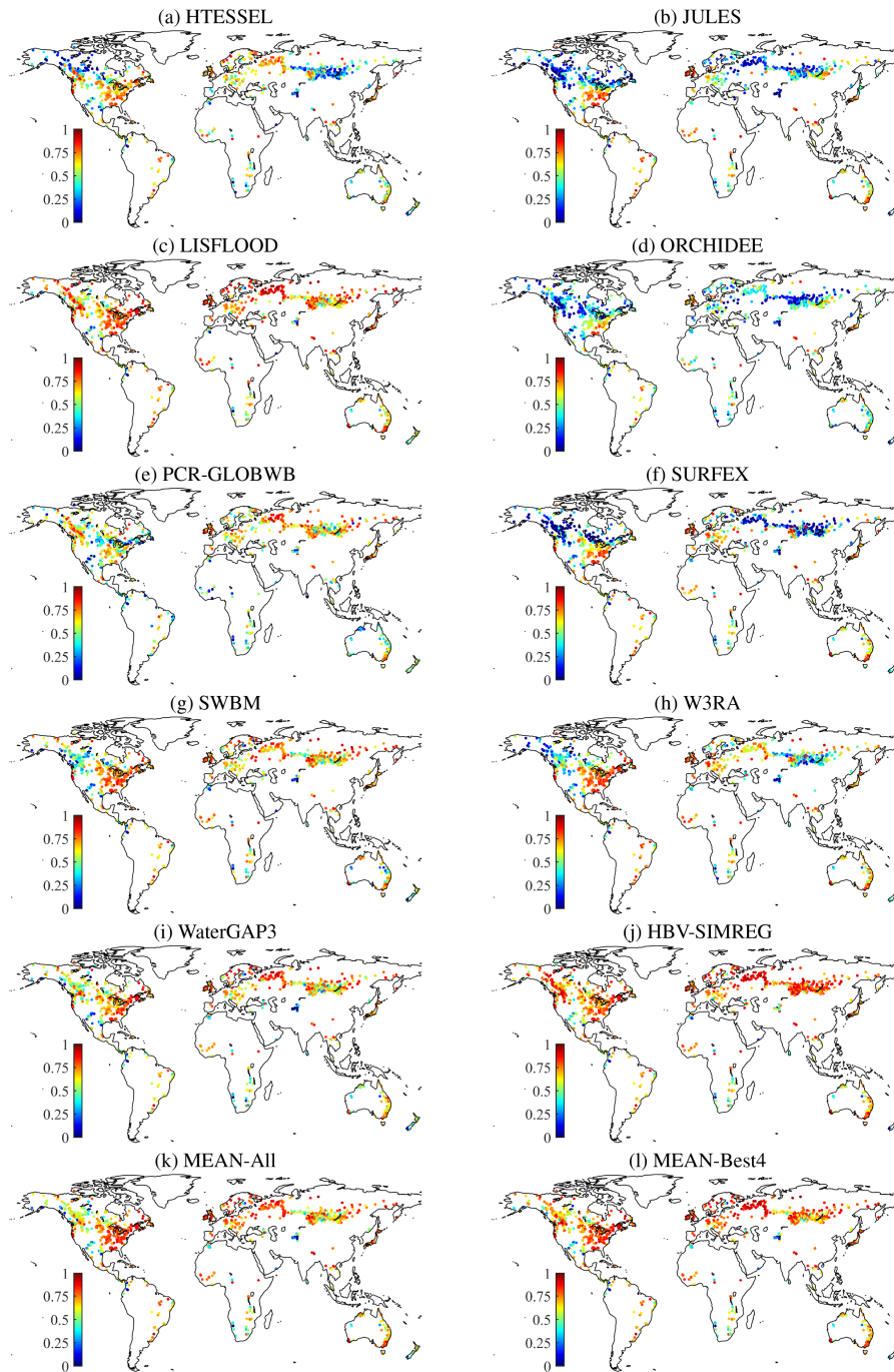
Figure 2. Correlation coefficients calculated between simulated and observed monthly runoff ( r_{\text{mon}} ; unitless) for the catchments. Each data point represents a catchment centroid ( n = 966 ).
