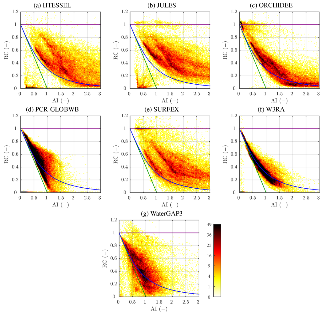
Figure 3. For the seven models with data on the available energy, density plots of grid cell values of aridity index (AI) versus runoff coefficient (RC). The green line represents the energy limit for which actual evaporation equals PET, the purple line represents the water limit for which runoff equals P , whereas the blue line represents the Budyko (1974) curve.
