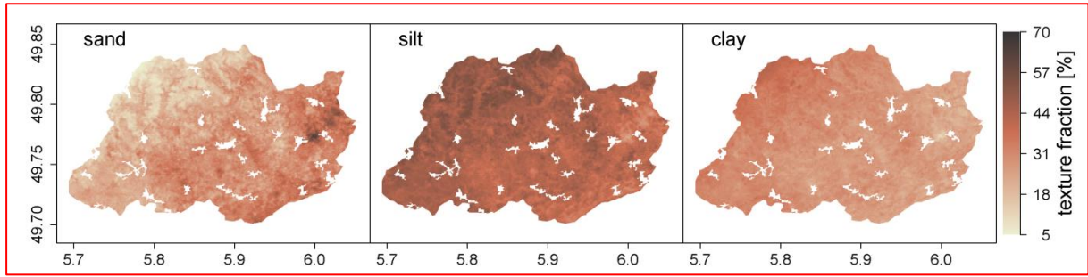
Figure 8: Exemplary mean value maps of soil texture fractions estimated with the CV50 CVS from the possible 212 different data sets. There are no significant differences between the different mean value maps for the different CVSs. Moreover, differences to the maps based on the full sample set are minor (compare Fig. 7).
