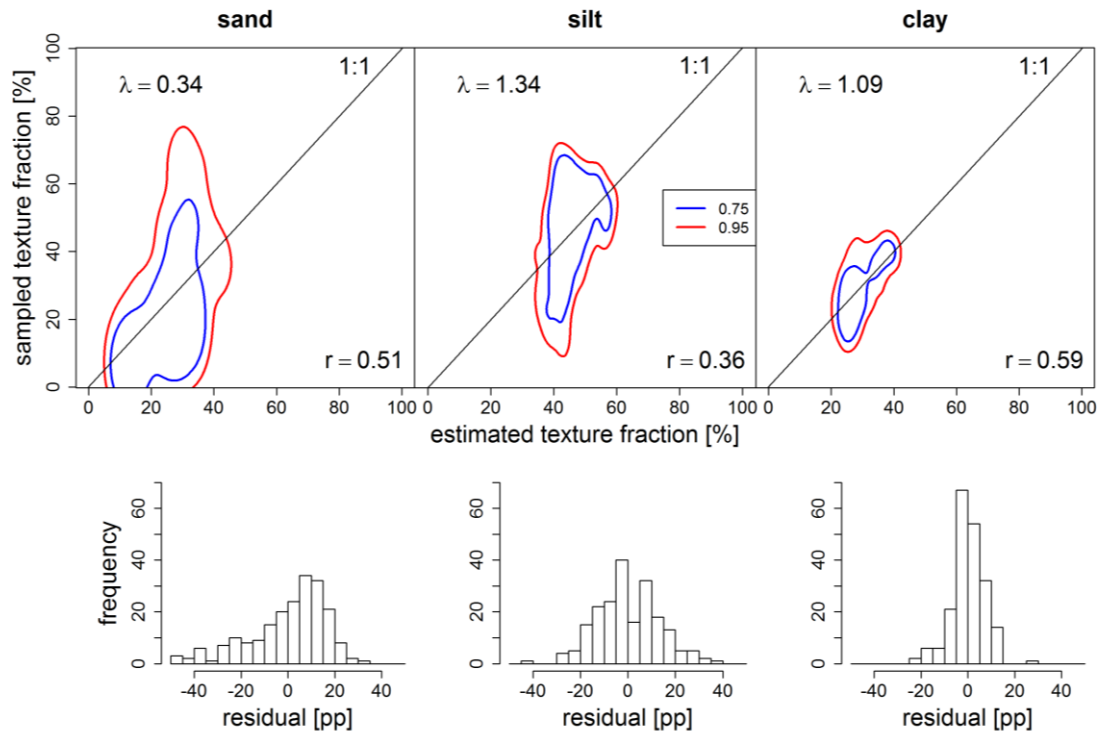
Figure 6. MLRE results for predicting sand, silt, and clay fractions estimated with three components of the PCA data. The distribution contours (upper panels) show the sampled versus the estimated texture data after BCT and sigmoidal capping. 95%- (red outline) and 75%-quantiles (blue outline) are shown. \lambda -values of the BCT (upper left) and Pearson correlation coefficient r between the sample and estimator data (lower right) are also noted. The lower panels show the respective distributions of residuals [estimator - data] and their skewness related to the BCT \lambda -values after back transformation.
