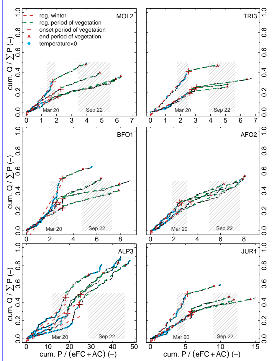
Figure 5. Type II dimensionless double mass curves for six catchments of different geological units. The \text{dDMCs-dDMC} depicted here are the same as those depicted in Fig. ??4 but with the difference that the abscissa is scaled using the sum of average effective field capacity (eFC) and air capacity (AC). All other properties are analogue to Fig. ??4.
