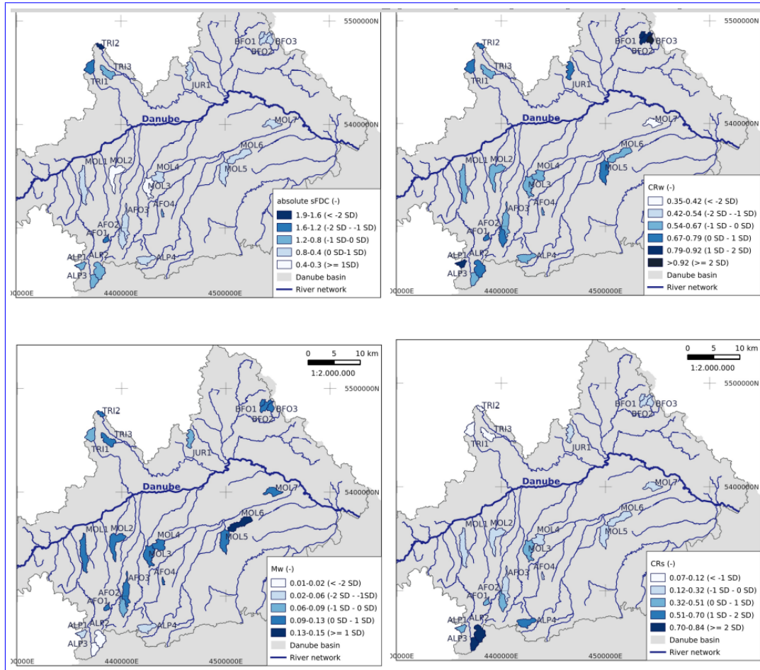
Figure 7. Seasonal- The panels show maps of a) absolute values of the slope of the flow duration curves for (sFDC) (-) (top left), b) winter runoff coefficients ( CR_w ) (-) obtained from the site AFO4. They exhibit considerable differences in type I dDMC (top right), c) the slopes between winter rate of how fast dimensionless relative release grows with the 33rd potential renewal rate of the soil stock ( m_w ) (bottom left panel) and 66th flow percentile d) summer runoff coefficients (dashed vertical lines CR_s ) which are widely used to characterise average flow conditions (Sawicz et al., 2011) (-) (bottom right panel). The vegetation and dormant period are separated using applied color code is derived from the temperature index method proposed by Menzel et al. (2003) standard deviation (SD) of each data set.
