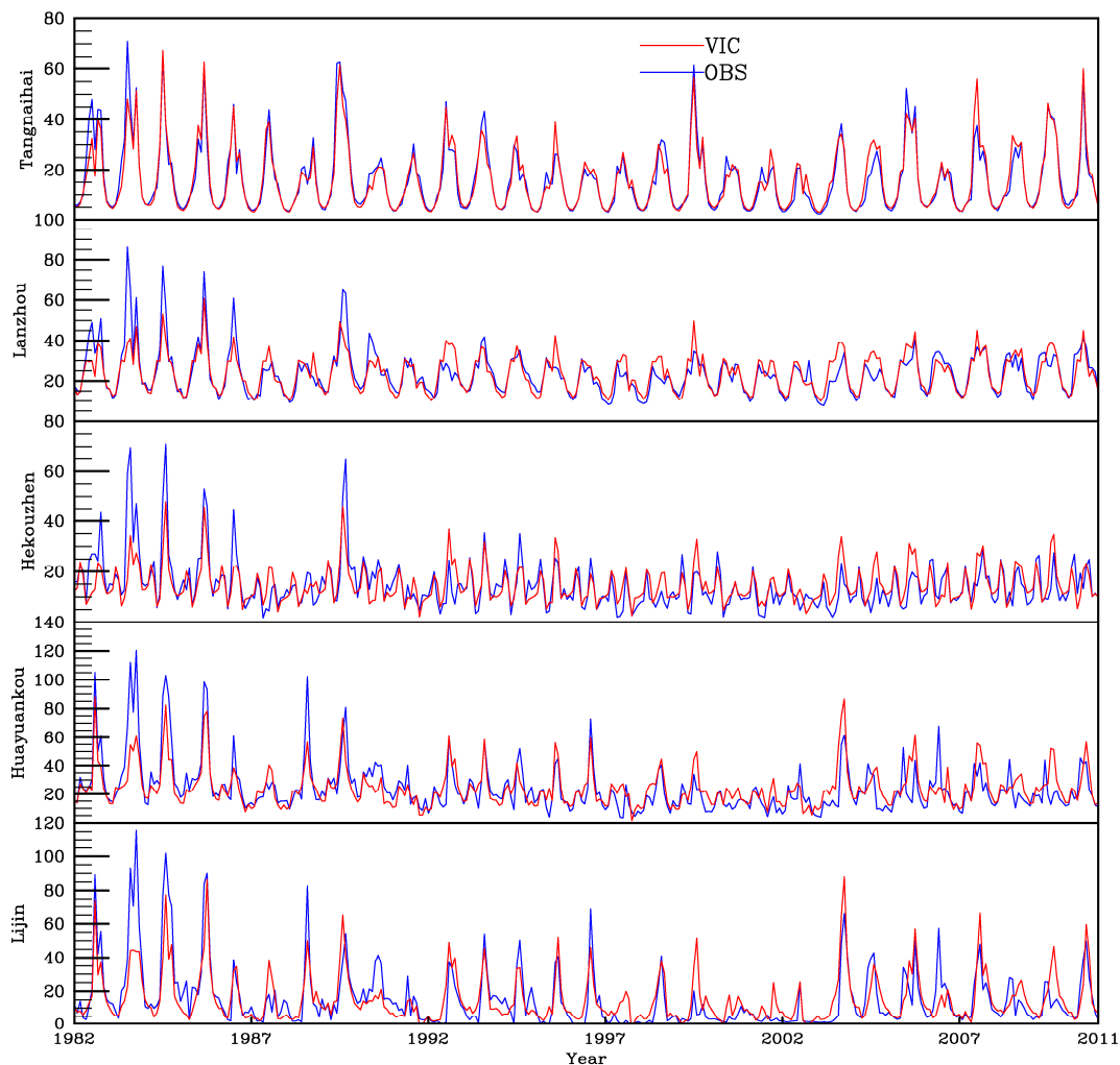
Figure 7. Observation (blue) and post-processed VIC simulation (red) for themonthly streamflow ( 10^8 \text{ m}^3/\text{s} ) at five hydrological gauges located from upper to lower mainstream of the Yellow River. During the post-processing procedure, the simulated streamflow without human interventions is linearly regressed against the observed streamflow for each target month.
