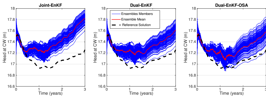
Figure 11. Reference (dashed) and predicted (solid) hydraulic head evolution at the control well: CW. Results are obtained using the Joint-EnKF, Dual-EnKF and the Dual-EnKF OSA schemes with 100 members, 1 day as observation frequency, 25 observation wells, and 0.50 m of measurement noise. The last 18 months are purely based on the forecast model prediction with no assimilation of data.
