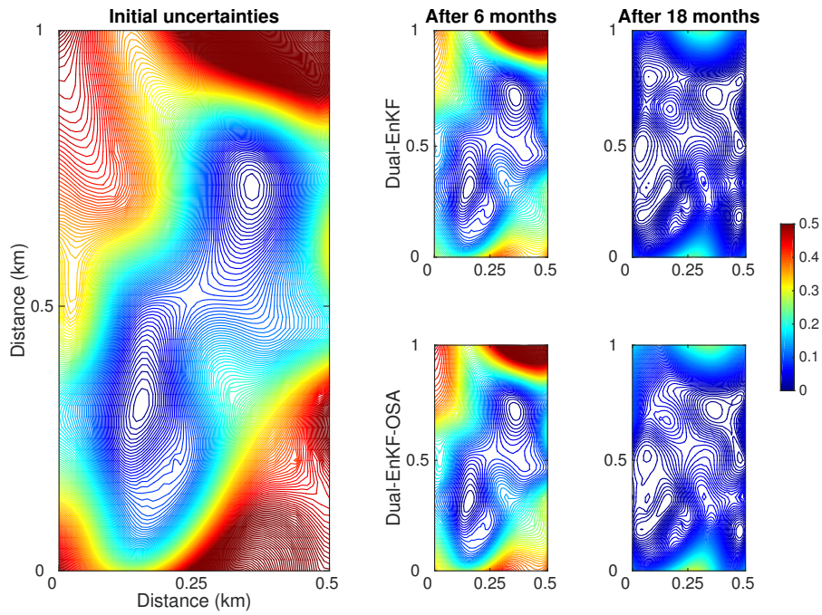
Figure 10. Left panel: Ensemble variance map of the initial conductivity field. Right sub-panels: Ensemble variance maps of estimated conductivity after 6 and 18 month assimilation periods using the Dual-EnKF and the proposed Dual-EnKF OSA schemes. These results are obtained with 100 members, 5 days of observation frequency, 9 observation wells, and 0.10 m as measurement noise.
