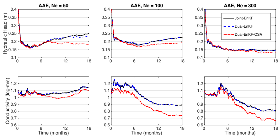
Figure 4. AAE time-series of the hydraulic head and conductivity using the Joint-EnKF, Dual-EnKF and Dual-EnKF OSA . Results are shown for 3 scenarios in which assimilation of hydraulic head data are obtained from nine wells every 0.5 days. The three experimental scenarios use 50, 100 and 300 ensemble members with 0.50 m as the measurement error.
