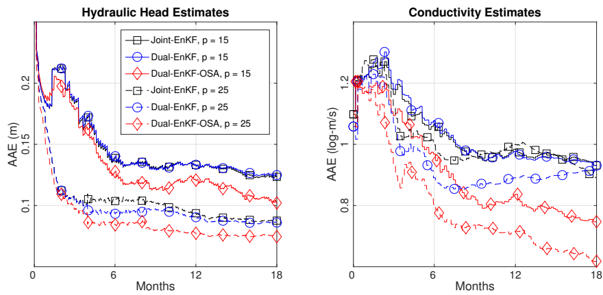
Figure 7. Time series of AAE of hydraulic head (left panel) and conductivity (right panel) using the Joint-EnKF, Dual-EnKF and Dual-EnKF OSA schemes. Results are shown for 2 scenarios in which assimilation of hydraulic head data are obtained from 15 and 25 wells (uniformly distributed throughout the aquifer domain) every 5 days. The four experimental scenarios use 100 ensemble members and 0.10 m as the measurement error standard deviation. The number of wells is denoted by p .
