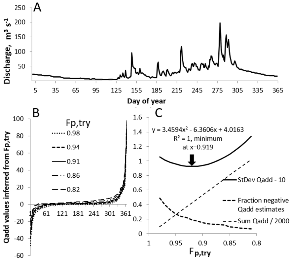
Figure 4. Example of the derivation of best fitting F_{p,try} value for an example hydrograph (A) (expressed as \text{m}^3 \text{s}^{-1} rather than \text{mm d}^{-1} as figures 2 and 3) on the basis of the inferred Q_a distribution (cumulative frequency in B), and three properties of this distribution (C): its sum, frequency of negative values and standard deviation; the F_{p,try} minimum of the latter is derived from the parameters of a fitted quadratic equation
