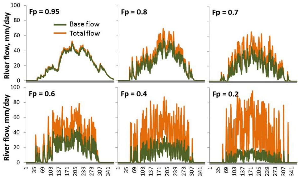
Figure 2. Example of daily river flow, split into a base flow and additional flow component, for a unimodal sinus-based rainfall probability multiplied with a rainfall depth calculated as 60^{\wedge}\text{rand}(0.1) mm/day (~120 rainy days, annual Q \sim 1600 mm) in watersheds characterized by F_p values ranging from 0.95 to 0.2
