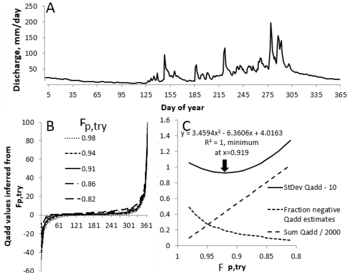
Figure 4. Example of the derivation of best fitting F_{p,try} value for an example hydrograph (A) on the basis of the inferred Q_a distribution (cumulative frequency in B), and three properties of this distribution (C): its sum, frequency of negative values and standard deviation; the F_{p,try} minimum of the latter is derived from the parameters of a fitted quadratic equation
