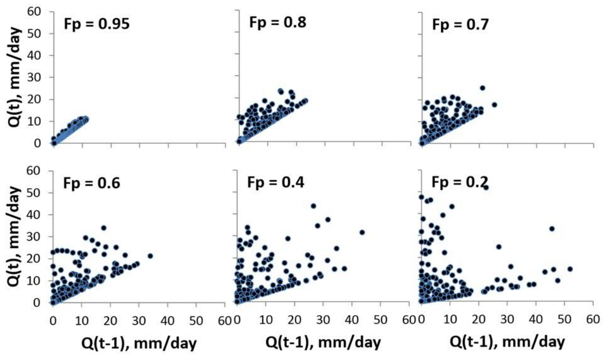
Figure 3. Biplots of Q(t) versus Q(t-1) for the same simulations as Figure 2
