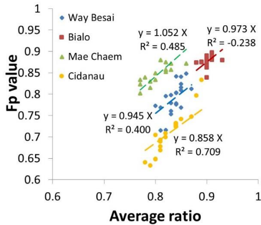
Figure 7. Comparison of yearly data for four watersheds (see paper II) analysed with common flow separation methods (as in Fig. 6) and the flow persistence method
