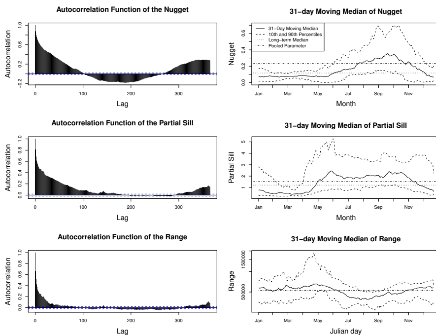
Figure 6. Autocorrelation function and 31-day moving median of daily variogram parameters.
