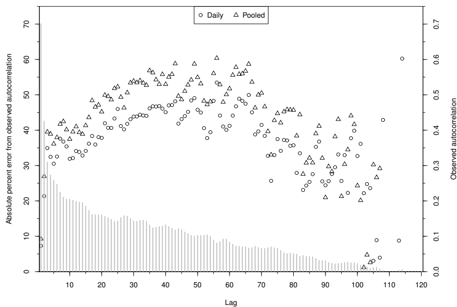
Figure 5. Absolute percent error between observed and estimated autocorrelation of daily streamflows for estimates from both daily and pooled variograms (left-hand, vertical axis). The vertical bars, quantified on the right-hand, vertical axis, describe the observed autocorrelation as a reference.
