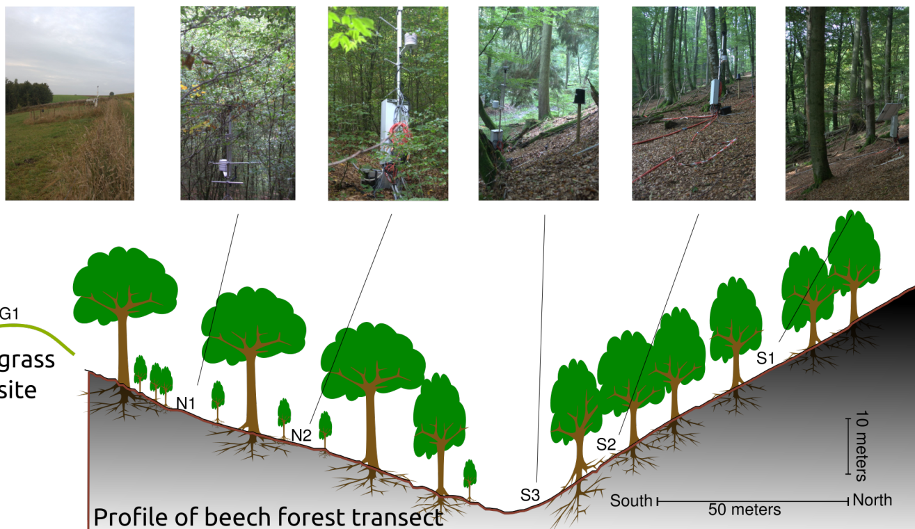
Figure 1. Measurement setup along a hillslope transect. Capital letters indicate aspect of the sites (N north-facing, S south-facing) and the numbering represents the position of the site on the hillslope: upslope (1), midslope (2) and downslope (3).
