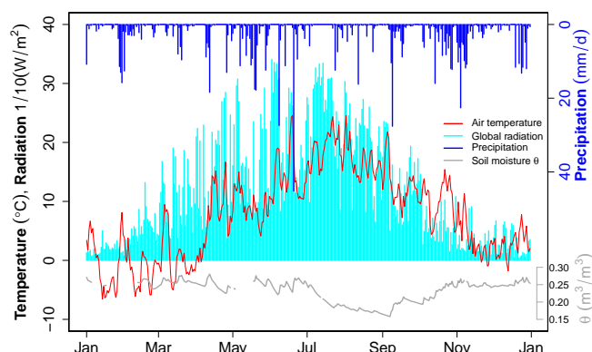
Figure 4. Meteorological forcing and average soil moisture at the grassland site (G1) for 2013. A few data gaps were filled with data from nearby grassland sites.
