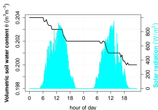
Figure 3. Observed diurnal decline in soil moisture over two sunny days in summer 2013 to illustrate the approach to estimate daily root water uptake from diurnal soil moisture variations. E_{RWU} is estimated at sensor level per day as a cumulative sum of differences from sunrise to sunset, in the absence of any nighttime variations or daytime increases in soil moisture.
