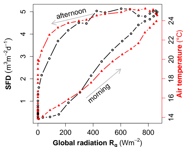
Figure 8. Hysteresis of sap flux density (left y-axis) and air temperature (right y-axis, red) plotted as a function of global radiation at the field site G1. Data are half-hourly values over one sunny summer day 2013-07-07. Sap flow data is taken from a beech (tree 1) at site S1.
