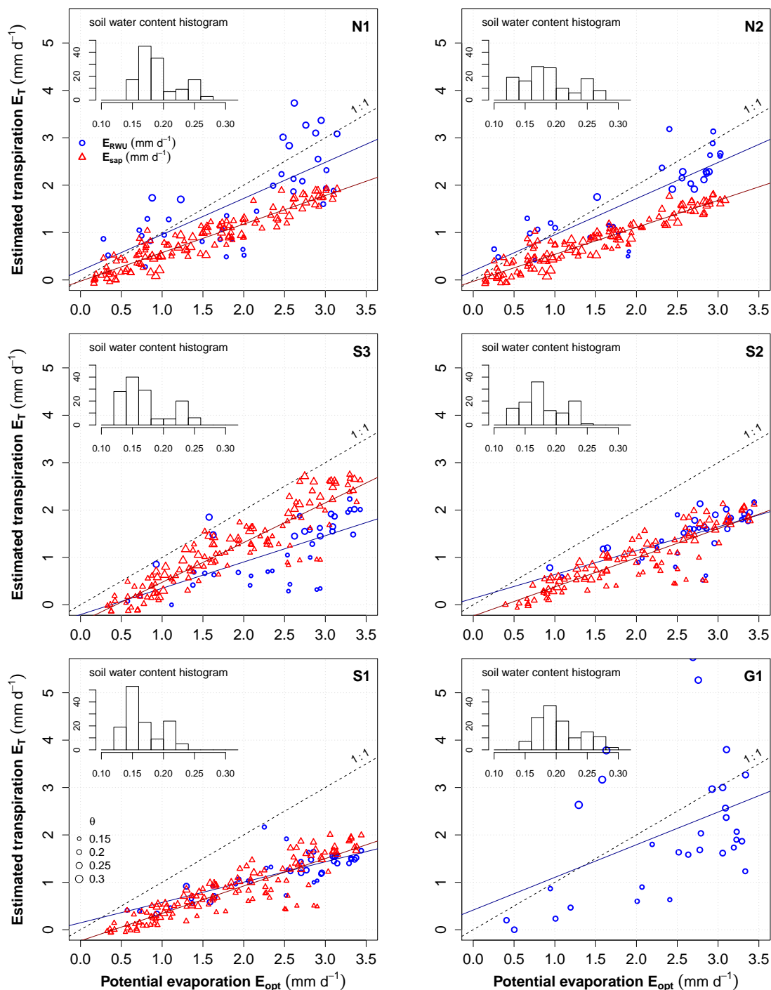
Figure 6. Site-average E_{RWU} (blue circles) and E_{sap} (red triangles) as function of E_{opt} during vegetation period (10.June - 20.October) in 2013. Each panel presents data of one site (see Figure 1 for site identifiers). The size of the symbols corresponds to the daily average soil moisture content. The histogram shows the distribution of site-average soil moisture. Solid lines depict the linear regression as tabulated in Table 2.
