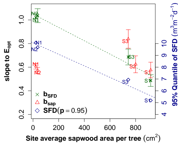
Figure 7. Sensitivity to E_{opt} as a function of the site-average sapwood area per tree computed by A_s/n_{tree} . On the left y-axis: sensitivity of site-average sap flux density b_{SFD} (green crosses, see also Table 3) and the sensitivity of the upscaled transpiration estimate b_{sap} (red triangles). The vertical bars show the standard deviation of the sensitivity estimates tabulated in Table 2 and 3. Right y-axis: 95% quantile of daily SFD maxima per site to estimate a robust maximum SFD . The dashed lines show linear regression model fits.
