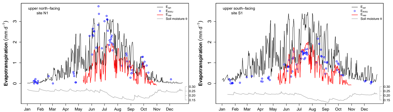
Figure 5. Time series of evapotranspiration estimates for north-facing hillslope site N1 in the left panel and south-facing site S1 in the right panel. E_{opt} is the potential evaporation derived from maximum power, E_{RWU} (blue points) and E_{sap} are transpiration estimates.
