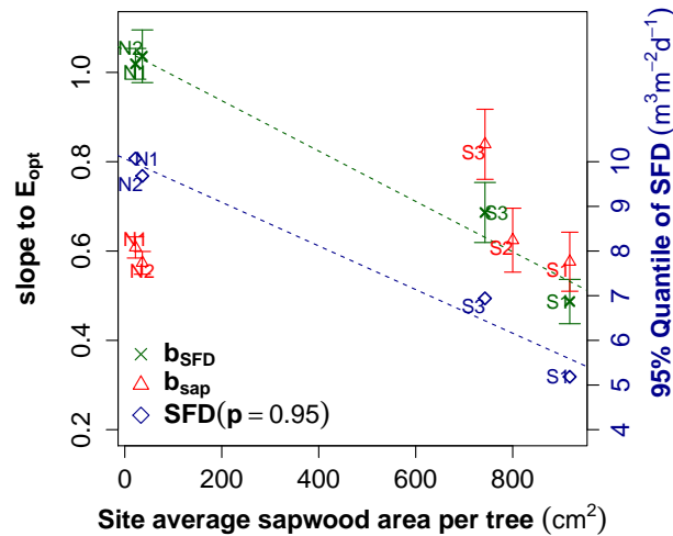
Figure 7. Sensitivity to E_{opt} as a function of the site-average sapwood area per tree computed by A_s/n_{tree} . On the left y-axis: sensitivity of site-average sap flux density b_{SFD} (green crosses, see also Table 3) and the sensitivity of the upscaled transpiration estimate b_{sap} (red triangles). The vertical bars show the standard deviation of the sensitivity estimates tabulated in Table 2 and 3. Right y-axis: 95% quantile of daily SFD maxima per site to estimate a robust maximum SFD . The dashed lines show linear regression model fits.
