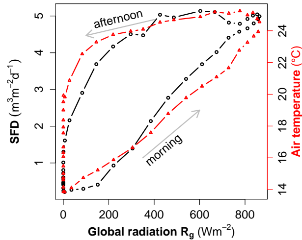
Figure 8. Hysteresis of sap flux density (left y-axis) and air temperature (right y-axis, red) plotted as a function of global radiation at the field site G1. Data are half-hourly values over one sunny summer day 2013-07-07. Sap flow data is taken from a beech (tree 1) at site S1.
