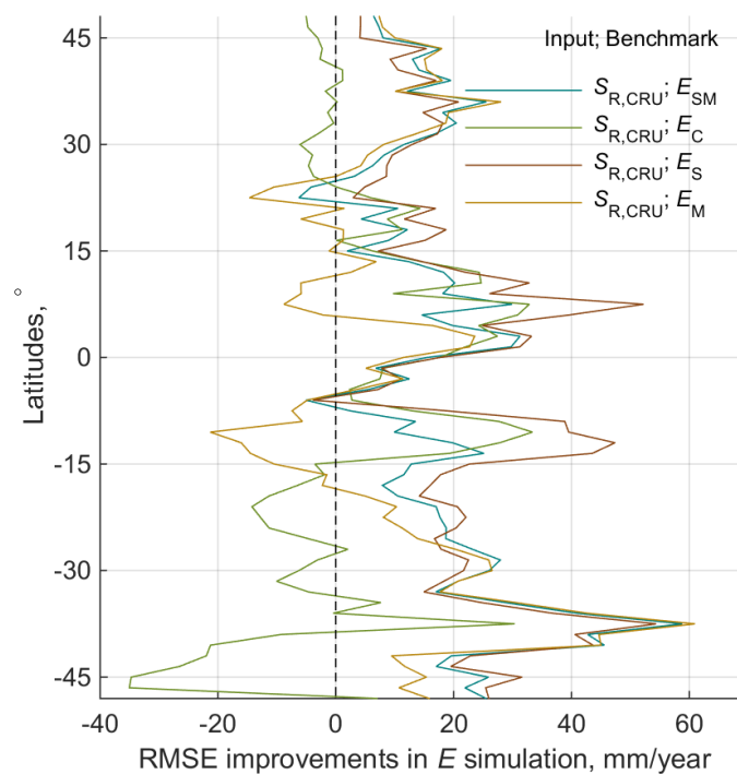
Fig. 1. Root mean square error improvements in STEAM evaporation simulation based on S_{R,CRU}:E_{SM} when using various E data as benchmark reference.
