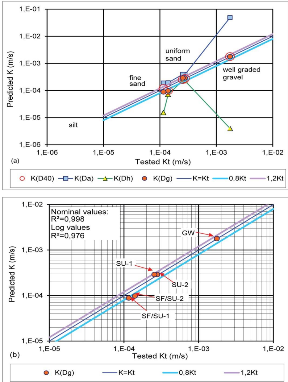
2 Figure 11. Graphical correlation between predicted K and tested K_t for sandy and gravelly aquifers. (a) 3 Difference between arithmetic, geometric and harmonic mean grain size, (b) Results of correlation 4 between predicted K(D_g) and tested K_t
