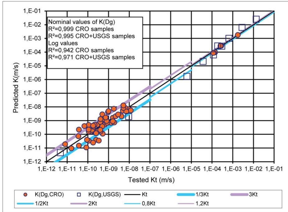
2 Figure 14. Verification of graphical and numerical correlation between the tested K_t and the predicted 3 hydraulic conductivity K(D_g) using referential geometric mean size for all samples
