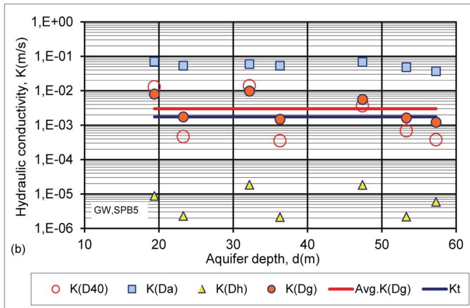
2 Figure 10. Predicted hydraulic conductivity calculated using KC equation for samples from gravely 3 aquifer (test field GW) – a) borehole SPB-3; b) borehole SP B-5
