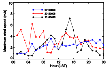
Figure 2. Time series of the 10min. maximum wind speed in one hour from Automatic Weather System located nearby PARSIVEL for three cases.
