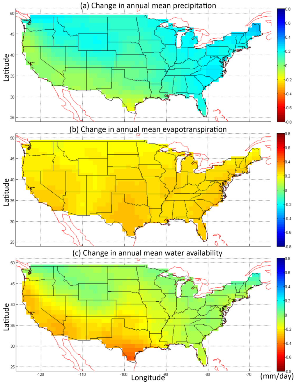
3 Fig. S-1 The change in the annual mean (a) P, (b) ET, and (c) P – ET over U.S. All units are 4 mm/day and the trend is defined as the average of 2030-2060 minus that of 1950-2005.
