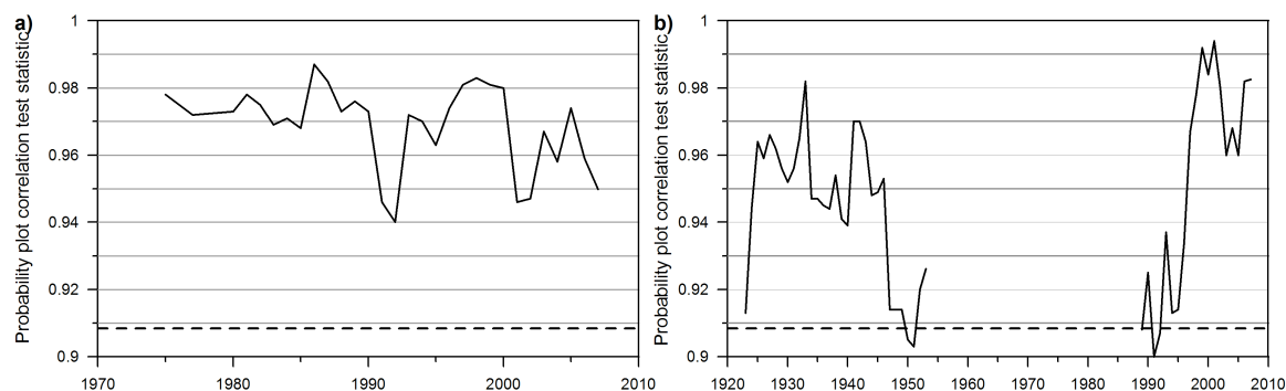
Figure 3: Results of the probability plot correlation test statistic (solid lines) for the 10-year moving window estimates of flood quantiles using the Gumbel distribution for Tarfala (a) and Abisko (b) catchment. The dashed line is indicating the lower critical value of the probability plot correlation test statistic of r=0.9084 for n=10 values and a significance level of 5% (Vogel, 1987).
