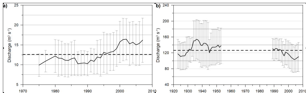
Figure 4: Time series of the mean and standard deviation (vertical error bars) of each 10-year moving window flood distribution.
