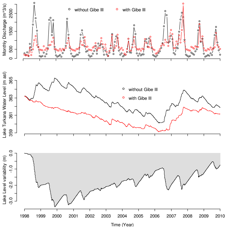
Fig. 3. Impact of the Gibe III dam evaluated using historical approach. Top panel: Total monthly Lake Turkana inflows; middle panel: the lake water levels; and bottom panel: the difference in lake levels; with (red line) and without (black line) the Gibe III dam. The model was run assuming the dam was commissioned on 1 January 1998.
