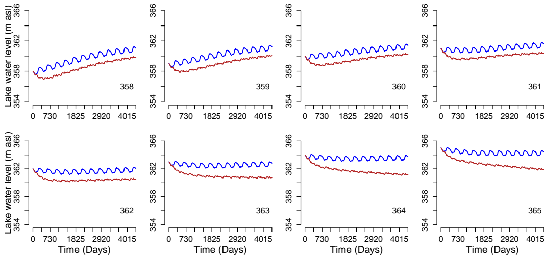
Fig. 6. Impact of the Gibe III dam on the Lake Turkana water levels simulated using the LLM approach and nonparametric bootstrap resampled (NBR) data. The impact of the dam is simulated for different initial lake levels from 358 m through 365 m a.s.l., shown on the y-axis. The x-axis shows time (days after the commencement of the dam). The blue line indicates lake level simulated without the dam; the dark red line indicates lake level simulated with the dam.
