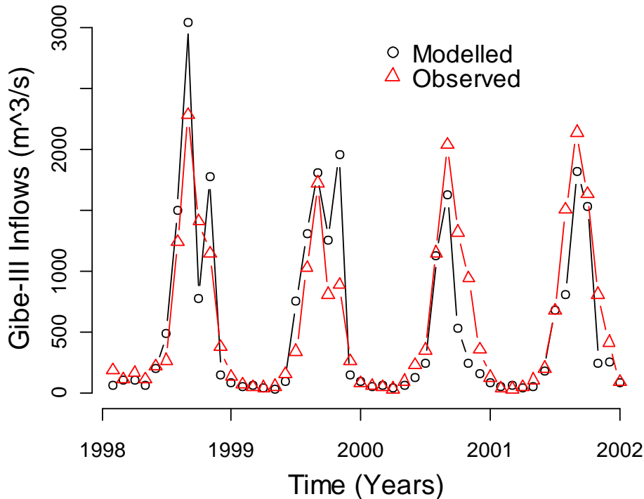
Fig. 2. Validation of modelled runoff data (after calibration) with observed monthly inflows (1998–2001) at the Gibe III dam site obtained from EEPCo (2009). Model calibrated using mean monthly streamflow data (1964–2001).
