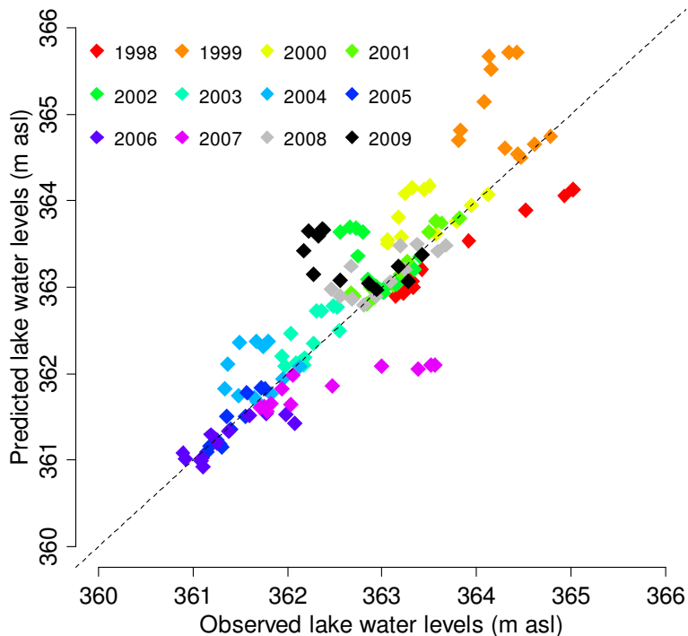
Fig. 5. Cross-validation of lake levels forecasted using a nonparametric bootstrap resampling (NBR) technique. Lake levels are predicted for each year using data from other years. For example, lake levels for 2006 are predicted using data from 1998–2005 and 2007–2009. The dotted line is the 1:1 line.
