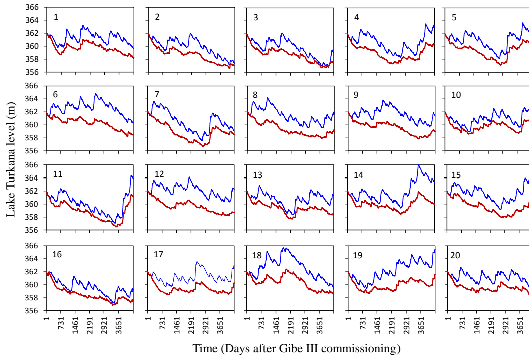
Fig. 4. Impact of the Gibe III dam on Lake Turkana water levels assessed based on 20 knowledge-based rainfall scenarios. The blue line shows the lake level fluctuations under each scenario without the Gibe III dam, and the red line shows the lake level fluctuations after the commissioning of the Gibe III dam.
