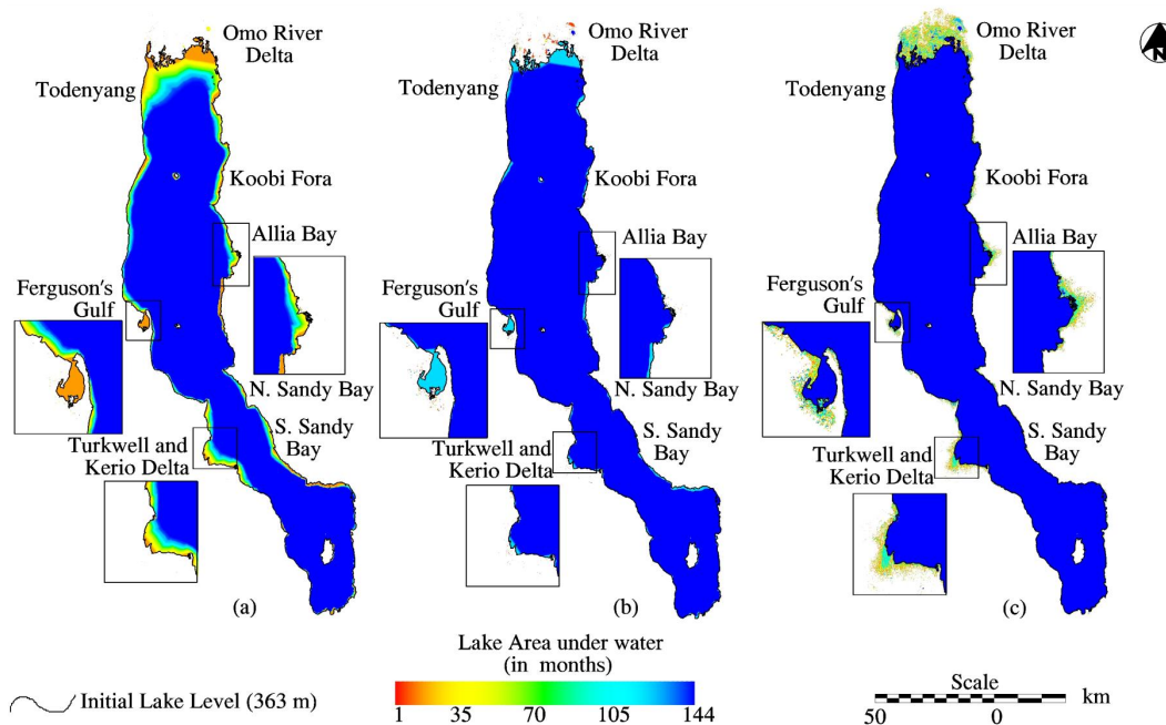
Fig. 8. Simulation of the impact of the Gibe III dam on Lake Turkana shoreline changes under three potential scenarios: (a) below normal rainfall scenario (lower 95 % confidence interval) – The lake shoreline would shrink up to 4 m inwards from the initial lake level (b) near normal rainfall scenario (median) – the lake shoreline would not show much variability from the initial lake level (c) above normal rainfall scenario (upper 95 % confidence interval) – the lake shoreline would grow outwards from the initial lake level, flooding several regions along the shoreline. The color denotes the time in months the lake is under water.
