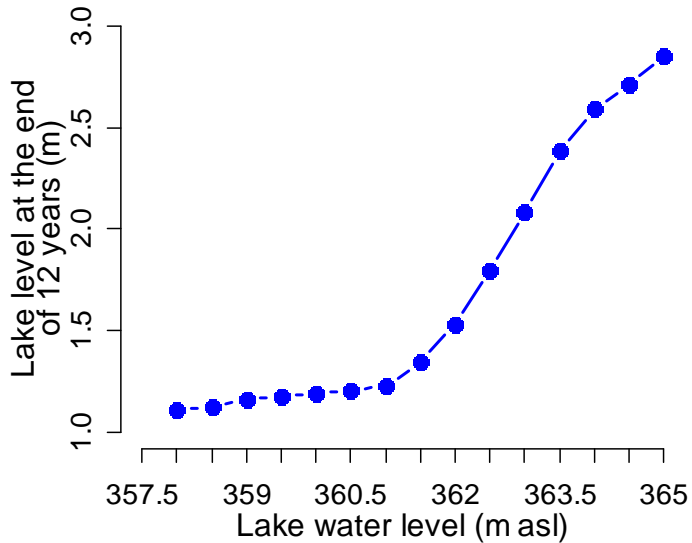
Fig. 7. Impact of the Gibe III dam (difference between with and without dam) at the end of 12 year simulation period is a function of initial lake level at the time of commencement of the dam.
