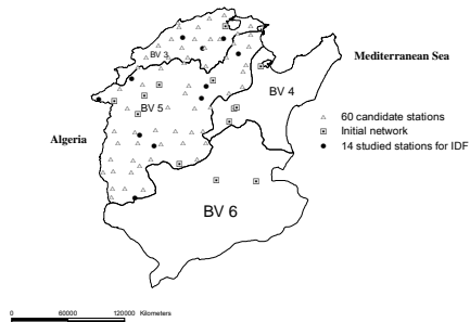
Figure 1. Location of rain gauges in the study area (Medjerda basin BV5 ; Northern coast basins BV3 and surrounding basins Meliane Basin BV4 ; Central Tunisia basins BV6 )
