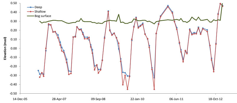
Figure 2: Comparison between the water level elevation in a shallow piezometer (screening 0.38 – 1.28 m below the surface) and a deep piezometer (screening 0.85 – 1.75 m below the surface) of a piezometer nest in a lagg swamp discharge zone in Burns Bog, Delta, BC.
