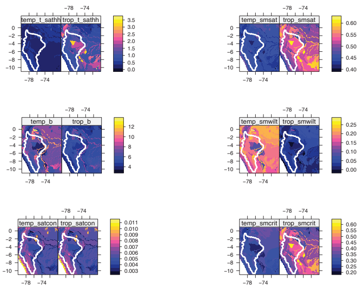
Fig. 2. Parameter variations generated using temperate (left panel) and tropical (right panel) pedotransfer functions in the topsoil (top 35cm). The hydraulic conductivity (mm/s) are unchanged
