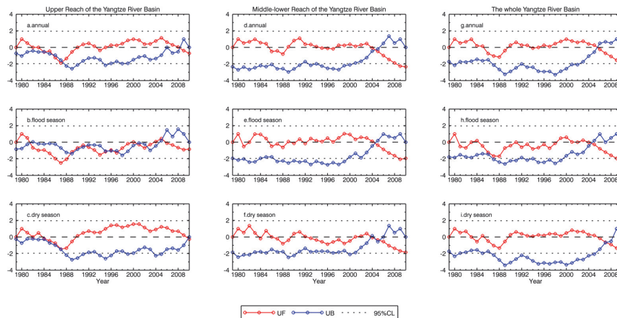
Fig. 7. The forward (UF) and backward (UB) Mann-Kendall statistic rank series for TWS standardized anomalies of annual ( a, d, g ), flood season ( b, e, h ) and dry season ( c, f, i ) during the period between 1979 and 2010 in upper reach, middle-lower reach and the whole Yangtze River basin, respectively (the horizontal dotted lines represent the critical values corresponding to the 95 % confidence level).
