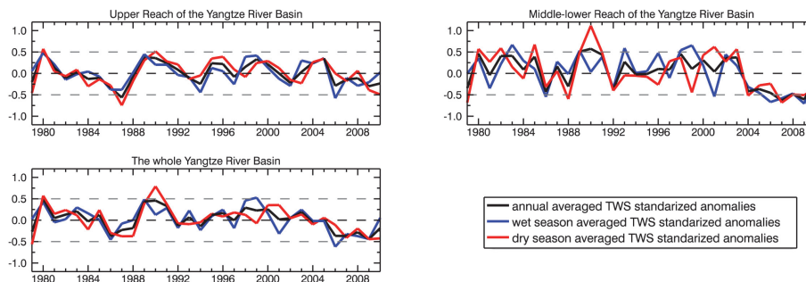
Fig. 8. The time series of the annual, wet season (May–October) and dry season averaged (November–April) TWS standardized anomalies in the upper, middle-lower Yangtze reach and the whole Yangtze River basin, respectively.
