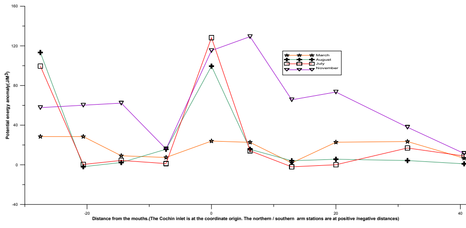
Fig. 1. Spatial variation in the potential energy anomaly (The months are characterised by south-west monsoon (July-August), north-east monsoon (November) and dry period (March))
