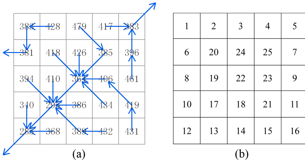
Fig. 1. DEM with depression removal algorithm applied and the relevant processing order
