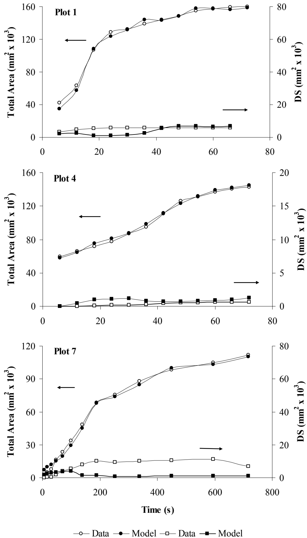
Fig. 5. The progression of overland flow A(t) and DS areas during the water inflow periods in three field plots as estimated from rectified video imagery and the model used in this study.
