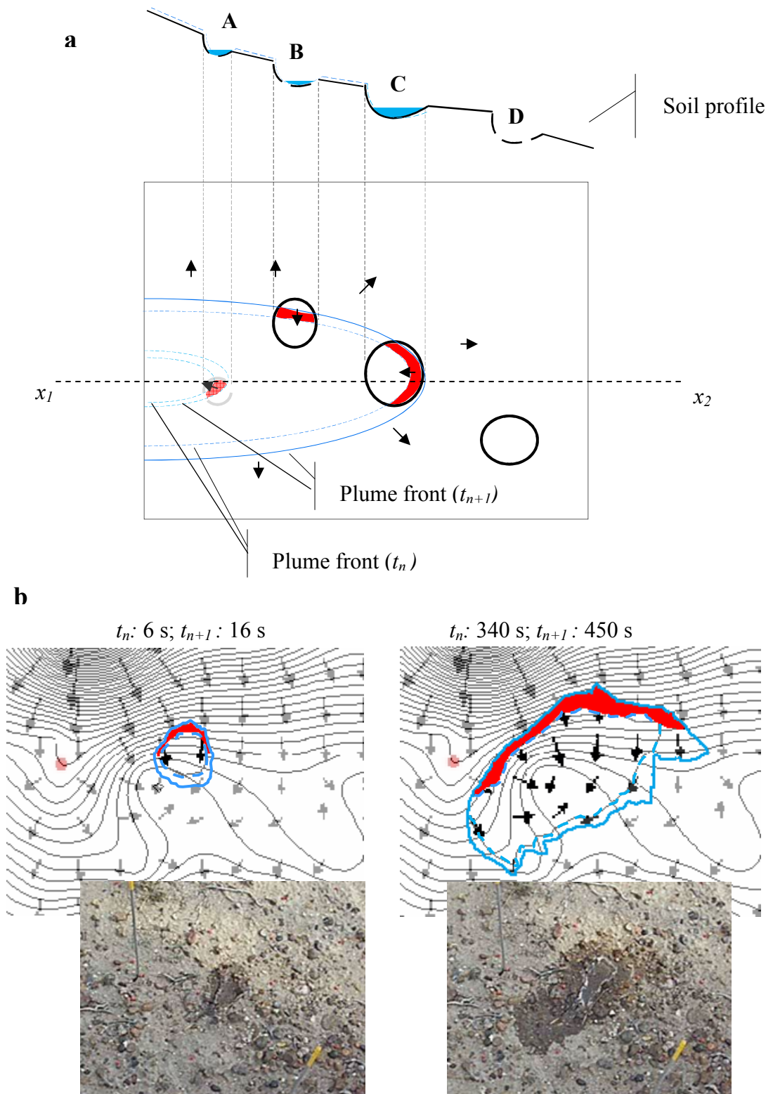
Fig. 2. Estimation of CSA (Counter-Slope-Advance) plume areas in this study. a. Local depressions (A-D) along a sloping soil profile at x_1 - x_2 . Advances of an overland plume up to depression C, over totally ponded A and partially ponded B-C. Part of the advances (red areas) were up-slope. b. Scene examples (lower insets) of plume advances at Plot #10 at two sampling intervals. Left t_n: 6\text{ s} , t_{n+1}: 16 ; right: t_n: 340\text{ s} , t_{n+1}: 450\text{ s} after water inflow start, overlaid on the plot DEM (contour interval: 1 mm) with DEM-based flow arrows.
