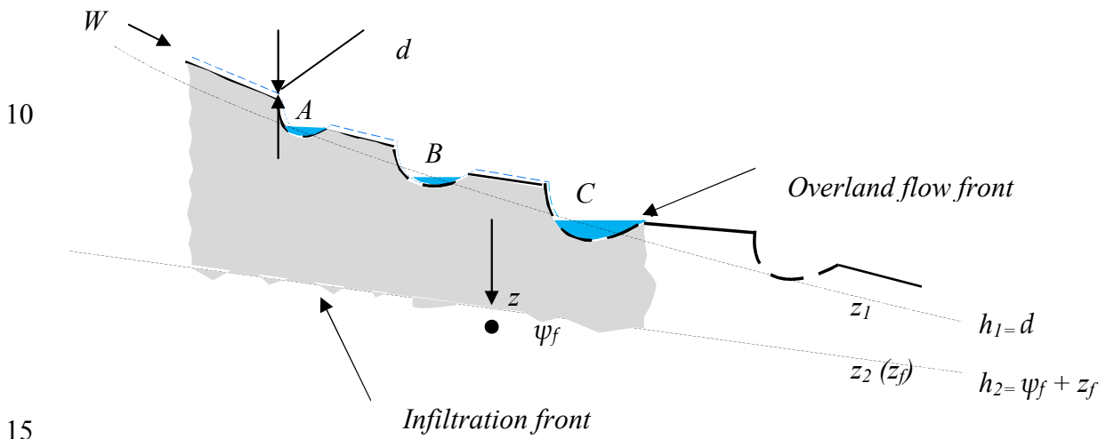
Fig. I-1. Schematic representation of parameters involved in considering infiltration up to depth z_f of a water inflow W on sloping soil with partially ponded depressed areas (A-C) (Also see main text, Figure 2).
