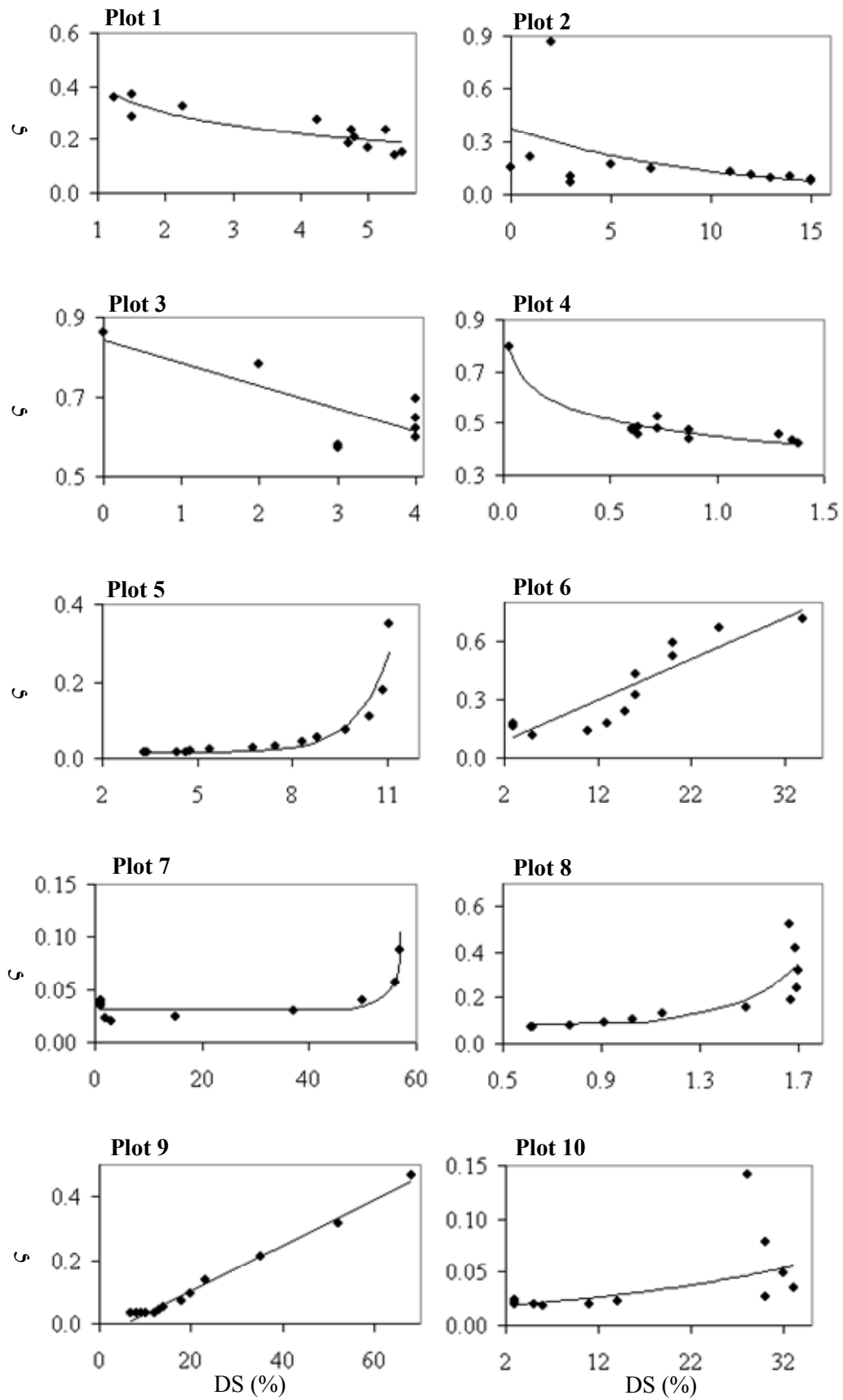
Fig. 6. Intra-plot time-series relations between the estimated DS and the runoff ( \zeta ) coefficient.
